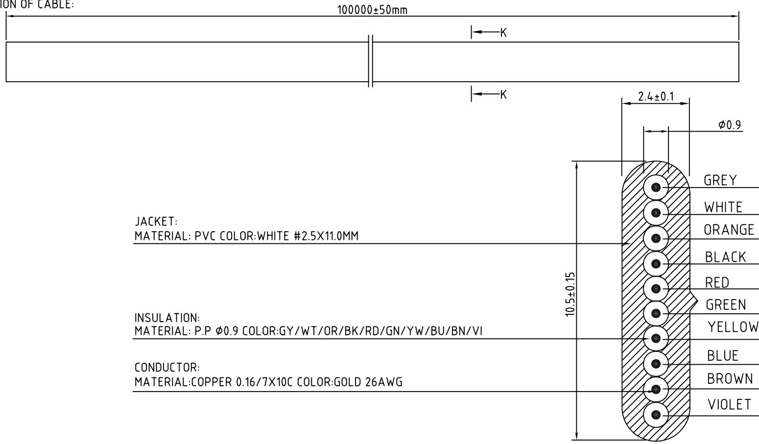
SECTION K-K
