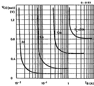
Collector-emitter Saturation Voltage (NPN types).
