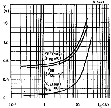
Base-emitter Voltage (PNP types).
