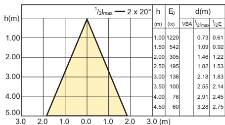
10-50W G53 AR111 WH 40D 3000K
