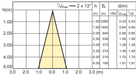
10-50W G53 AR111 WW 24D 2700K
