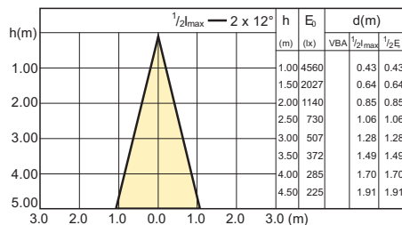
15-75W G53 AR111 WW 24D 2700K
