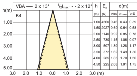
MASTER LEDspot LV AR111 15-75W G5.3 2700K 24D
