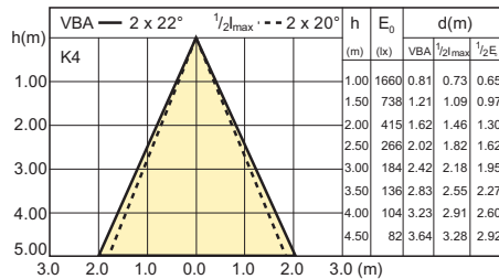
MASTER LEDspot LV AR111 15-75W G5.3 2700K 40D
