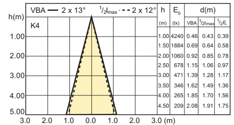
MASTER LEDspot LV AR111 15-75W GU10 2700K 24D
