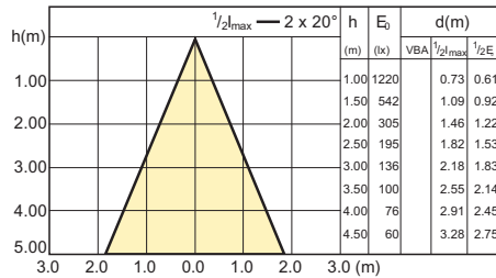
10-50W G53 AR111 WW 40D 2700K
