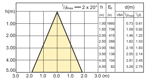
15-75W G53 AR111 WW 40D 2700K
