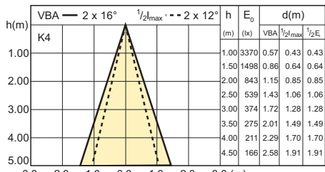
MASTER LEDspot LV AR111 10-50W G53 3000K 12V 24D
