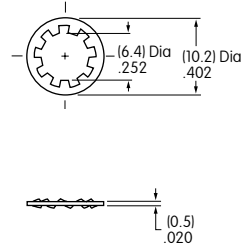
AT508 Lockwasher Steel with Zinc/Chrome (Not supplied with splashproof models)
