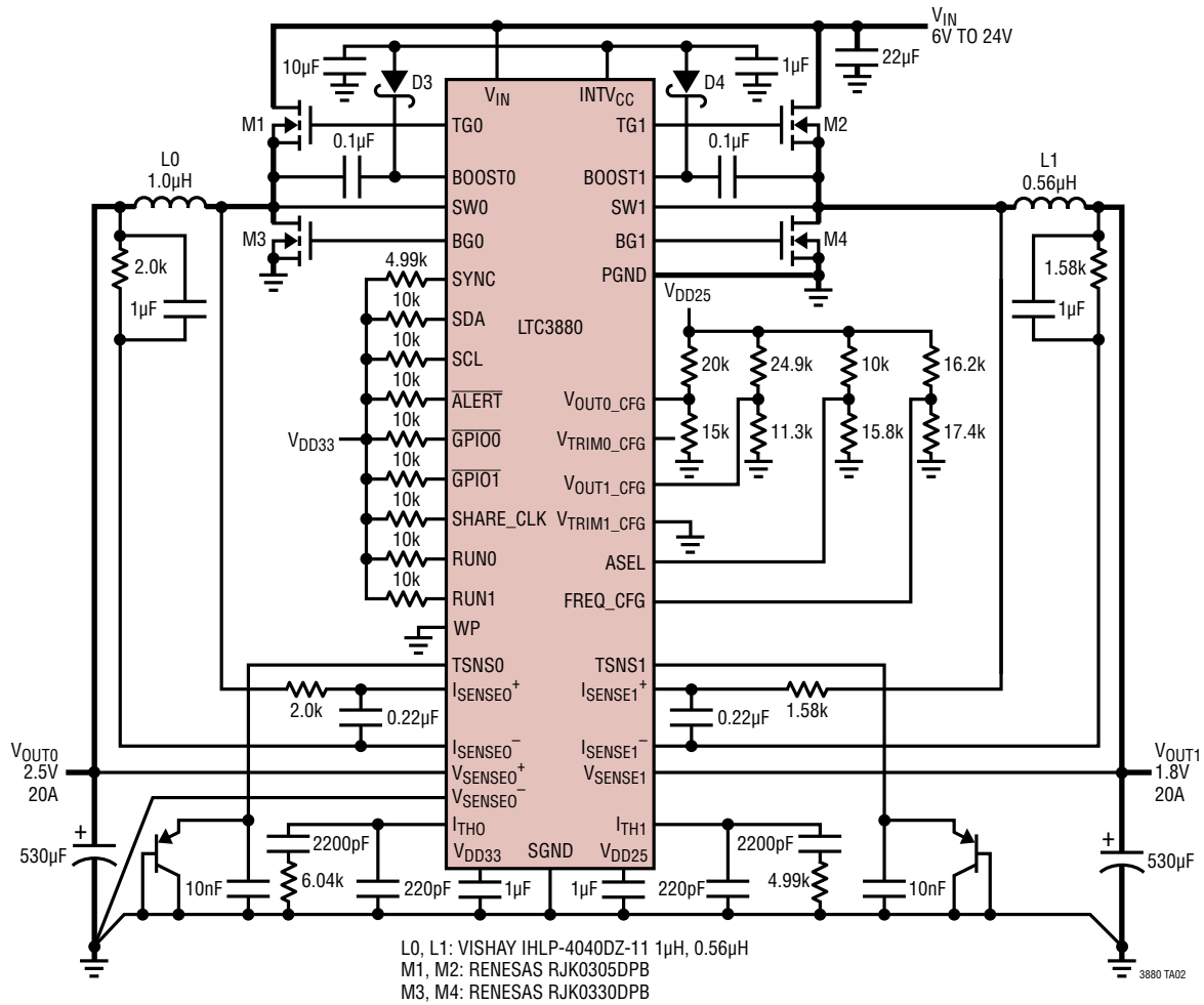
High Efficiency Dual 425kHz 2.5V/1.8V Step-Down Converter
