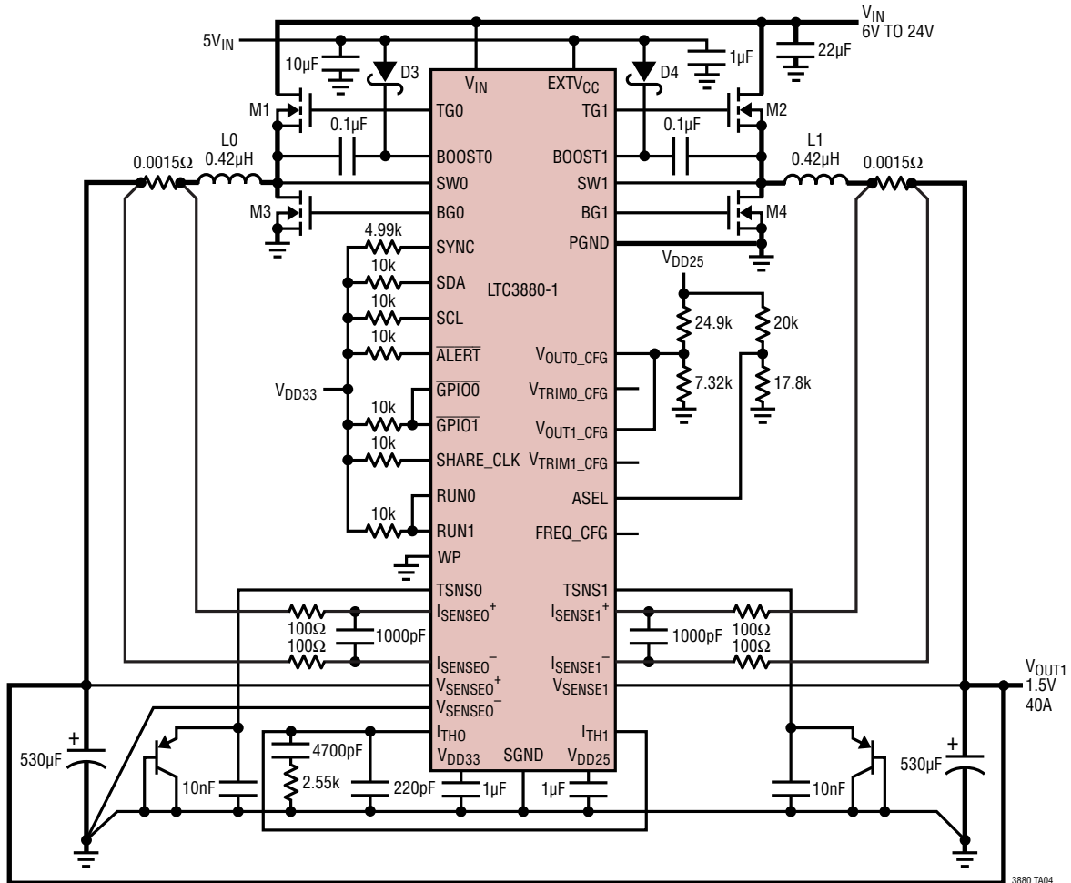
L0, L1: VITEC 59PR9875 0.42µH M1, M2: RENESAS RJK0305DPB M3, M4: RENESAS RJK0330DPB
