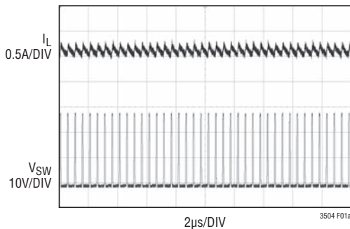
Figure 1a: The LT3504 Operating in Constant-Frequency Operation (Below V IN(PS) ), V IN = 26.5V, V OUT = 3.3V, f SW = 2MHz, t ON(MIN) = 74ns at T = 25°C
