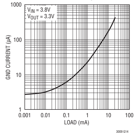
GND Pin Current vs I_{LOAD}
