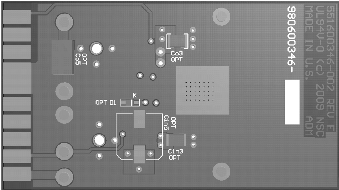
FIGURE 1. Top View and Bottom View of Evaluation PCB
