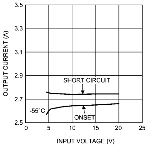
Current Limit 1.8V_{OUT} @ -55^\circ C
