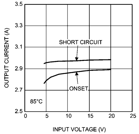
Current Limit 1.8V_{OUT} @ 85^\circ C
