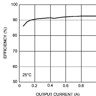
Efficiency V_{IN} = 12V V_{OUT} = 5.0V
