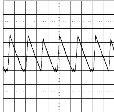
Transition Mode Operation V_{IN} = 12V, V_O = 3.3V, I_O = 0.29A
