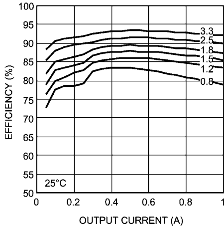
Efficiency 6V Input @ 25°C
