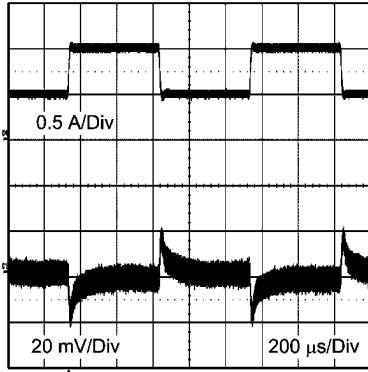
Transient Response 12V_{IN} 3.3V_O 0.6A to 1A Step
