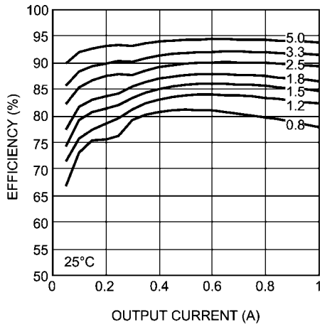
Efficiency 8V Input @ 25°C
