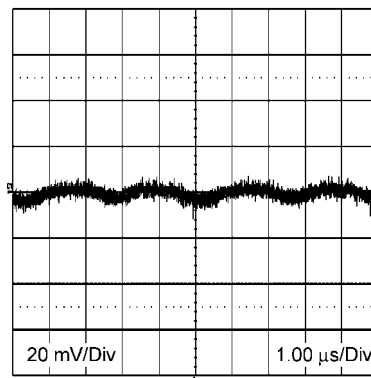
Output Ripple 12V IN 3.3V O 1A
