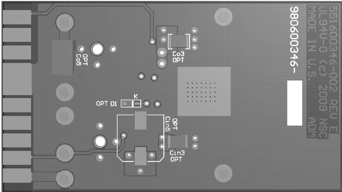
FIGURE 1. Top and bottom view of evaluation PCB
