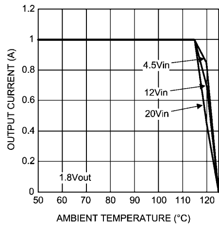
Thermal Derating V_{OUT} = 1.8V
