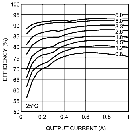
Efficiency 12V Input @ 25°C
