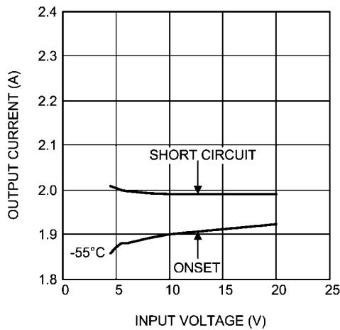
Current Limit 1.8V_{OUT} @ -55^\circ C
