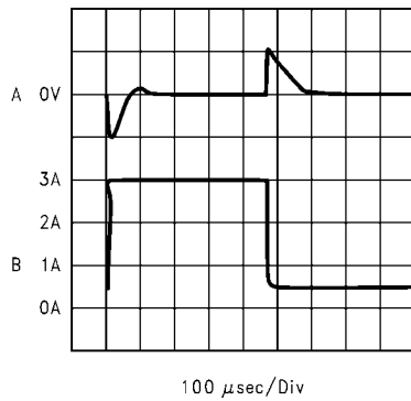
A: Output Voltage, 100 mV/div, AC-Coupled. B: Load Current: 500 mA to 3A Load Pulse Horizontal Time Base: 100 \mu s/div
