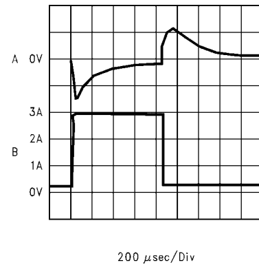
A: Output Voltage, 100 mV/div, AC-Coupled. B: Load Current: 200 mA to 3A Load Pulse Horizontal Time Base: 200 \mu s/div
