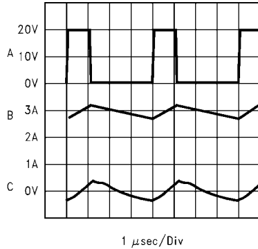
A: V_{SW} Pin Voltage, 10 V/div. B: Inductor Current, 1 A/div C: Output Ripple Voltage, 20 mV/div AC-Coupled Horizontal Time Base: 1 \mu s/div
