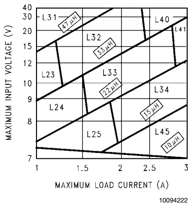
FIGURE 4. LM2670-5.0
