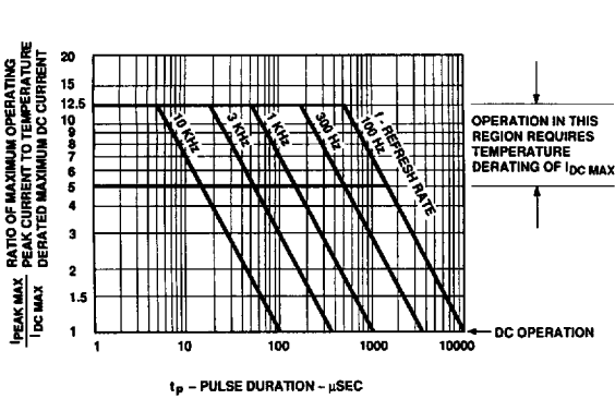
Figure 1. Maximum Tolerable Peak Current vs. Pulse Duration - Red.
