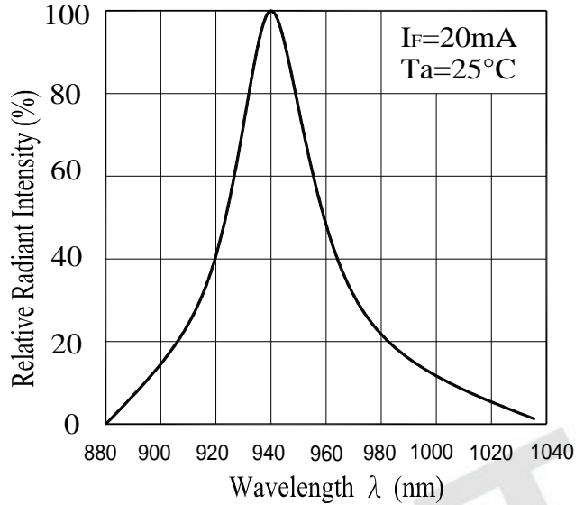
Fig.2 Spectral Distribution
