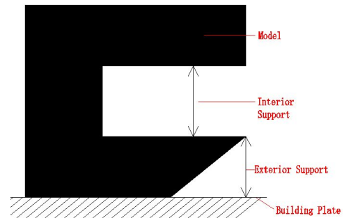
4.3.8.12 Structure of internal and external support of the model
