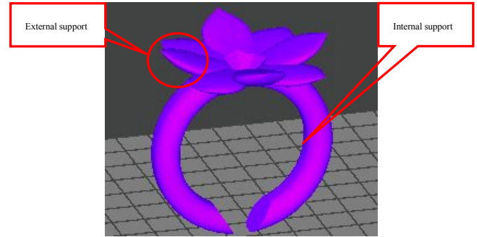
4.3.8.12 Structure of internal and external support of the model
