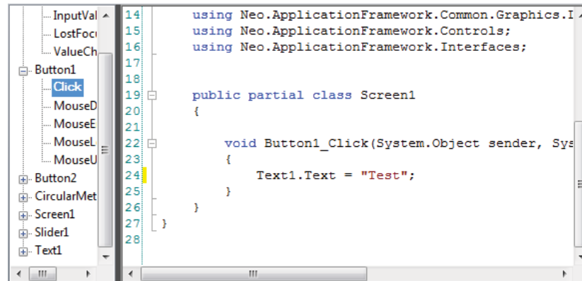
Highlight of an edited node in the tree view
