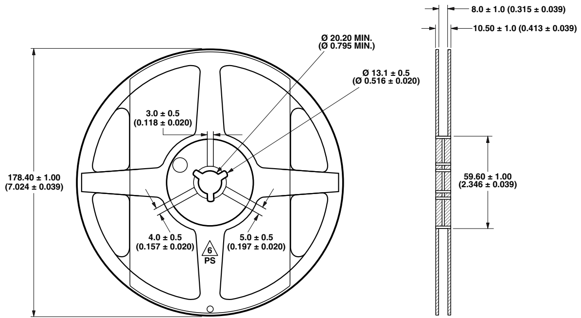
Figure 9. Reel Dimensions.
