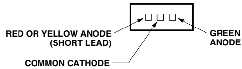
HLMP-08xx Straight Leads
