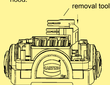
carrier hood
