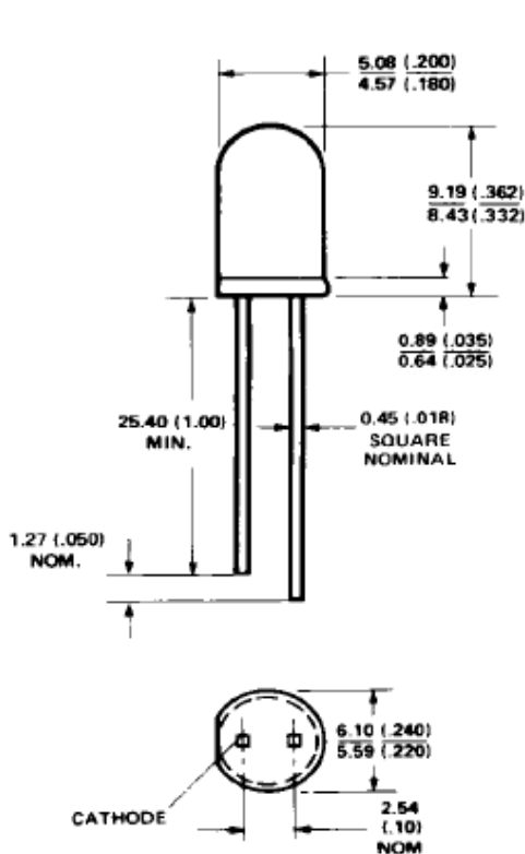
HLMP-4700, -4719, -4740 A
