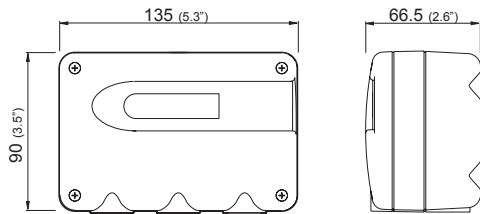
polycarbonate housing
