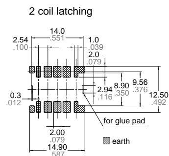
Tolerance: \pm 0.1 \pm .004
