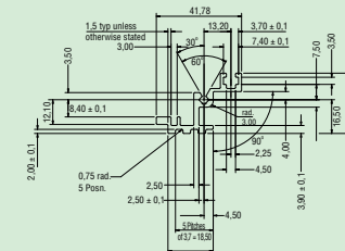
Handle Extrusion
