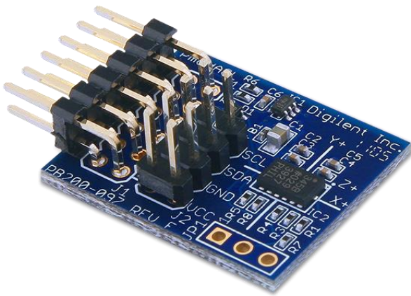
The PmodACL.
