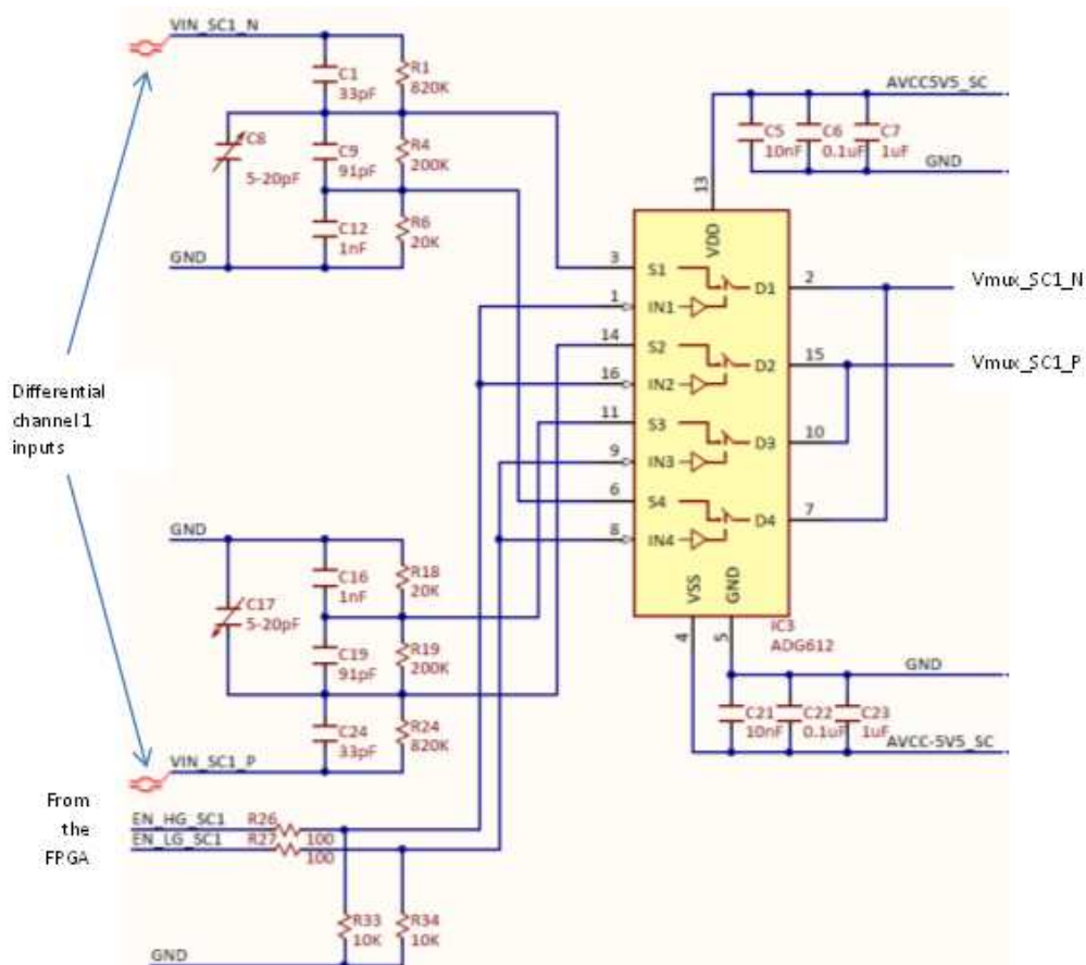
Figure 3. Input divider and gain selection. []
