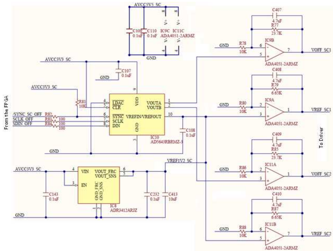
Figure 5. Scope reference and offset. □
