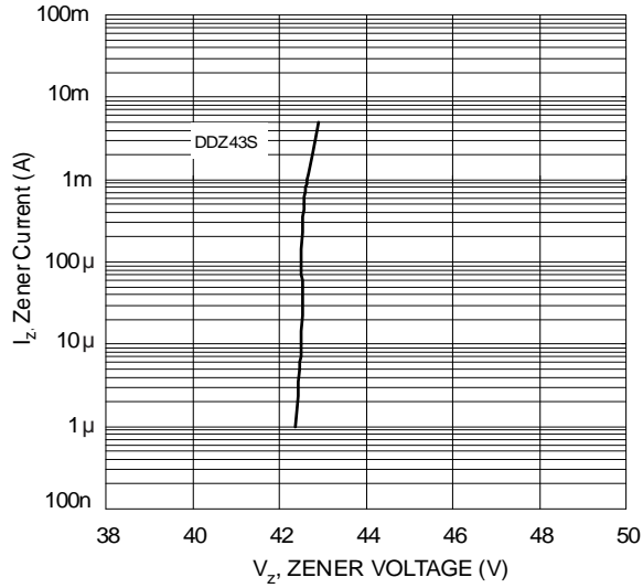
Fig. 5 Typical Zener Breakdown Characteristics, DDZ43S
