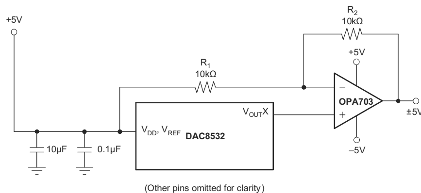
Figure 40. Bipolar Operation with the DAC8532
