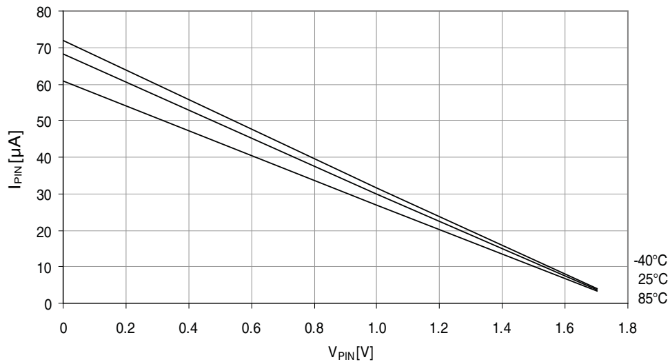
Figure 37-20. I/O pin pull-up resistor current vs. input voltage. V_{CC} = 1.8V .
