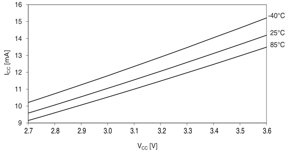
Figure 37-7. Active mode supply current vs. V_{CC} . f_{SYS} = 32\text{MHz} internal oscillator.
