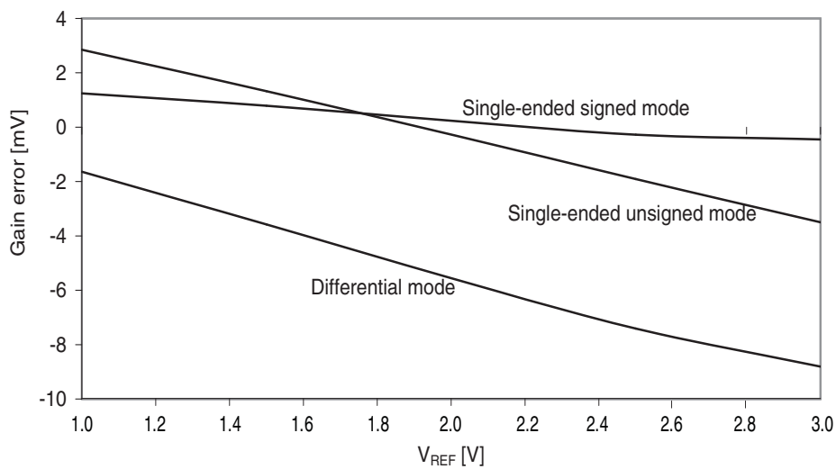
Figure 37-41. Gain error vs. V_{REF} . T = 25^{\circ}\text{C} , V_{CC} = 3.6\text{V} , ADC sampling speed = 500ksp/s.
