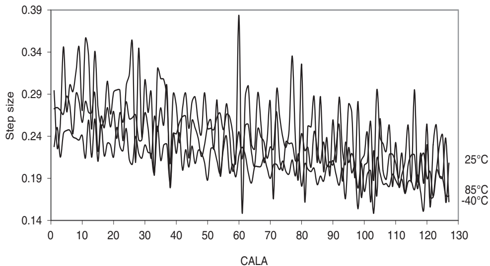
Figure 37-76. 32MHz internal oscillator CALA calibration step size.
