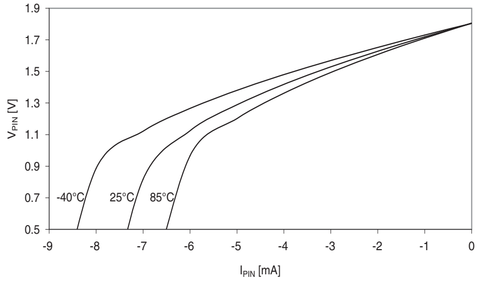
Figure 37-23. I/O pin output voltage vs. source current. V_{CC} = 1.8V .
