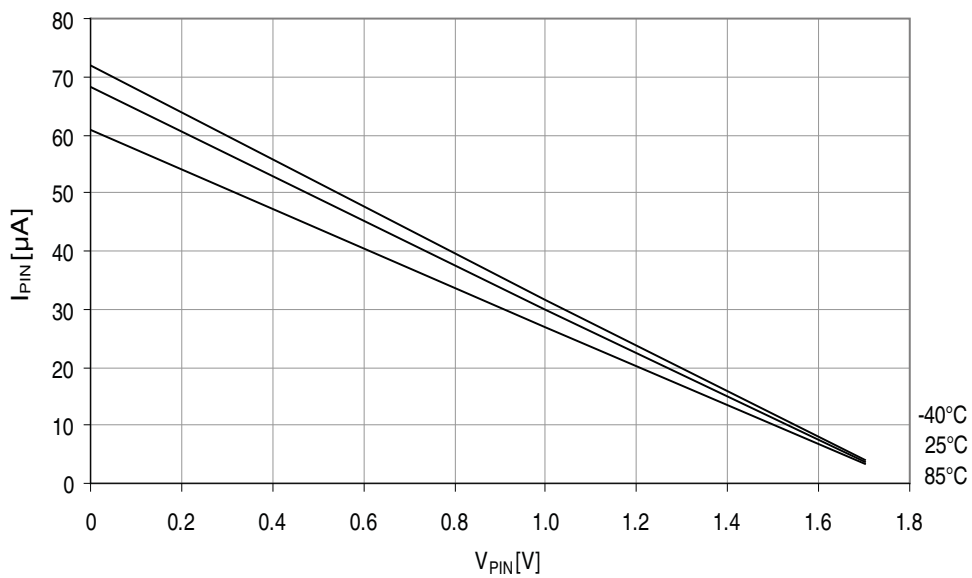
Figure 37-62. Reset pin pull-up resistor current vs. reset pin voltage.
