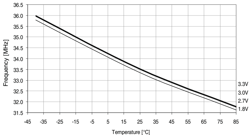
Figure 37-74. 32MHz internal oscillator frequency vs. temperature. DPLL disabled.
