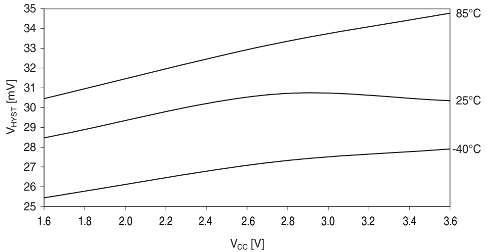
Figure 37-52. Analog comparator hysteresis vs. V_{CC} . Low power, small hysteresis.
