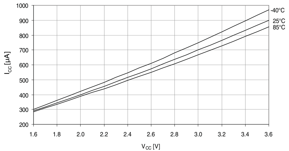
Figure 37-4. Active mode supply current vs. V_{CC} .
