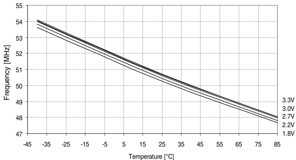
Figure 37-78. 48MHz internal oscillator frequency vs. temperature. DPLL disabled.
