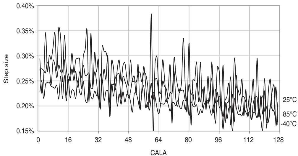
Figure 37-80. 48MHz internal oscillator CALA calibration step size. V_{CC} = 3.0V .
