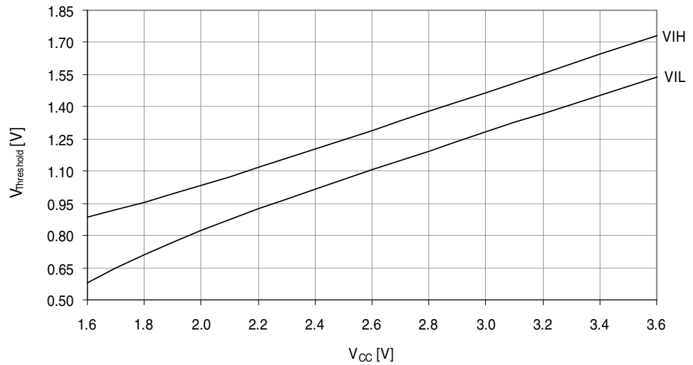
Figure 37-31. I/O pin input threshold voltage vs. V_{CC} . T = 25^{\circ}\text{C} .
