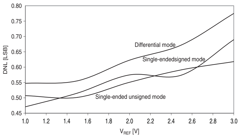
Figure 37-38. DNL error vs. external V_{REF} .
