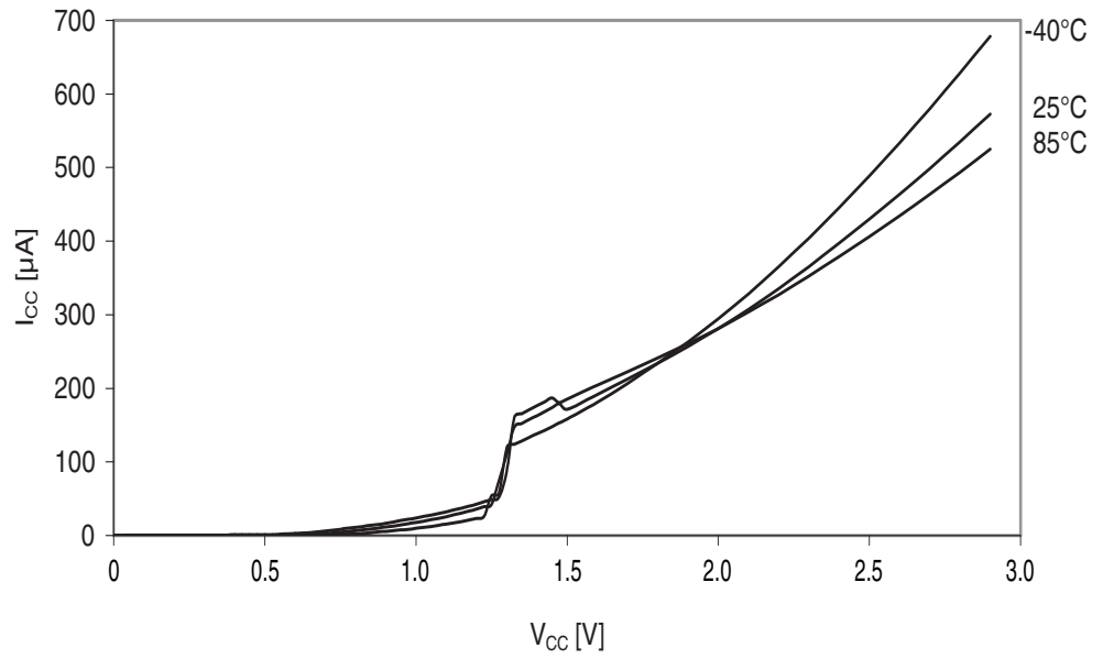
Figure 37-67. Power-on reset current consumption vs. V_{CC} . BOD level = 3.0V, enabled in continuous mode.
