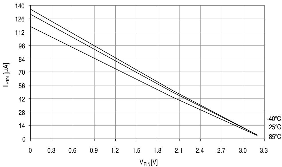
Figure 37-64. Reset pin pull-up resistor current vs. reset pin voltage. V_{CC} = 3.3V .
