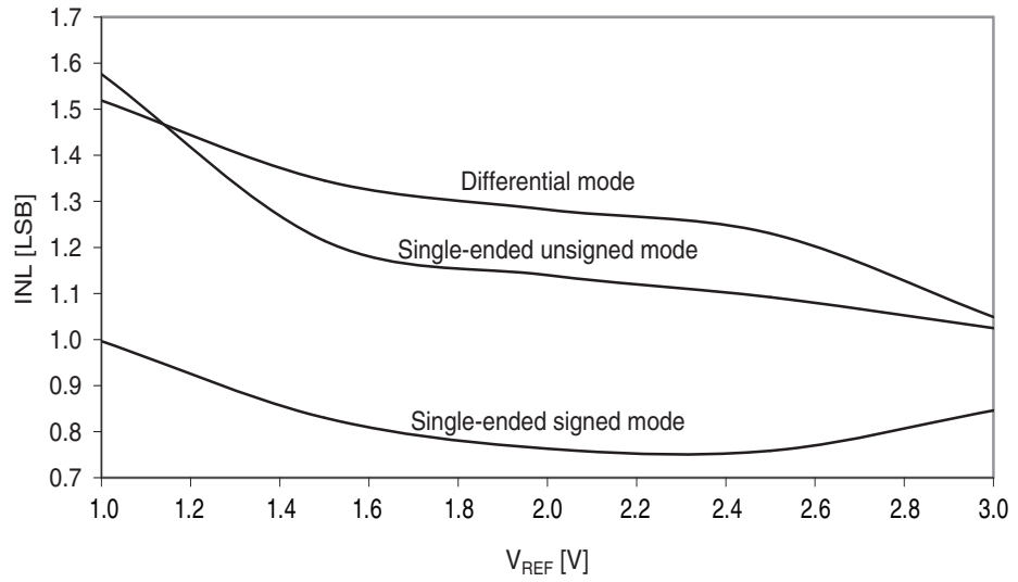
Figure 37-35. INL error vs. external V_{REF} . T = 25°C, V_{CC} = 3.6V , external reference.
