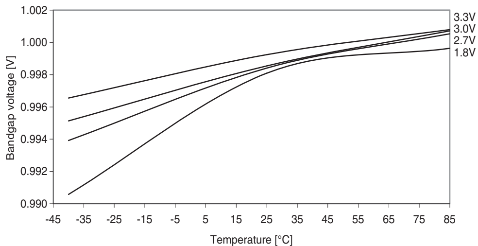
Figure 37-58. ADC/DAC Internal 1.0V reference vs. temperature.
