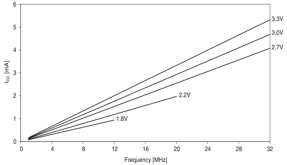
Figure 37-9. Idle mode supply current vs. frequency.
