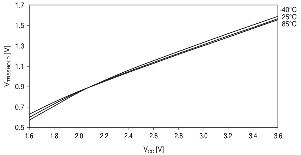
Figure 37-33. I/O pin input threshold voltage vs. V_{CC} . V_{IL} I/O pin read as "0".
