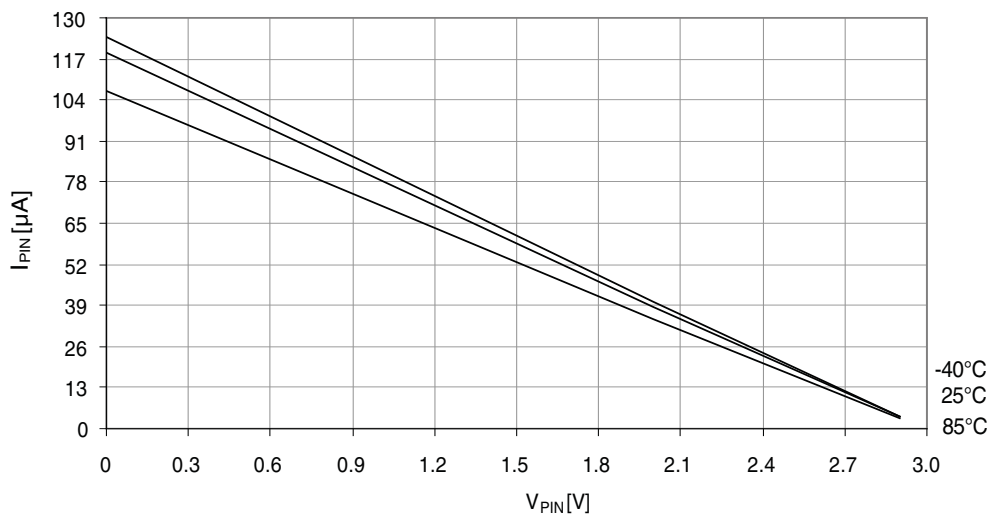
Figure 37-21. I/O pin pull-up resistor current vs. input voltage.
