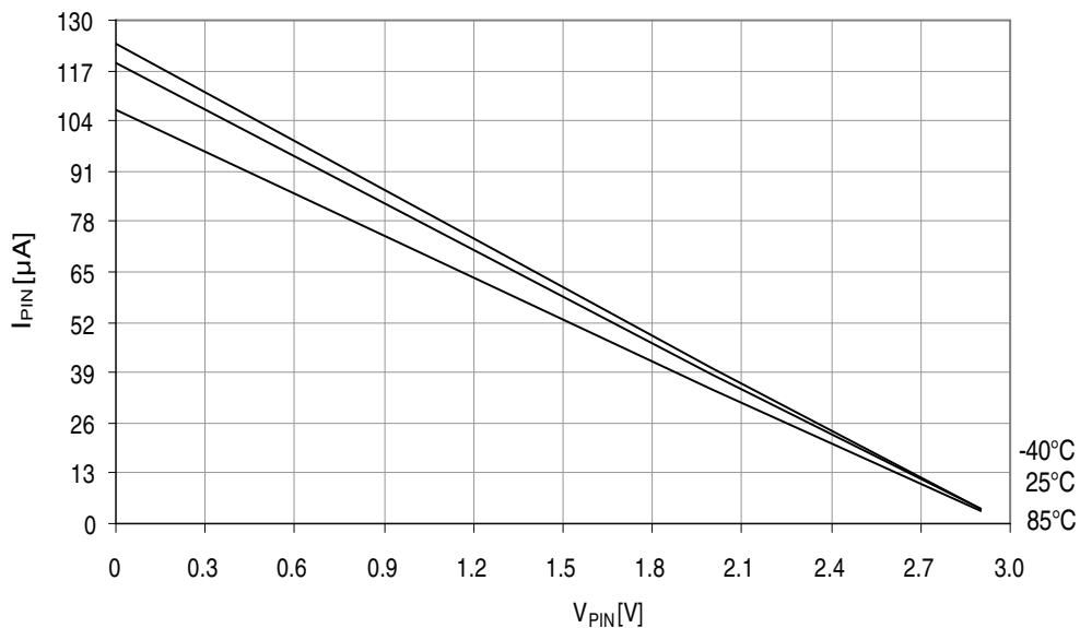
Figure 37-63. Reset pin pull-up resistor current vs. reset pin voltage. V_{CC} = 3.0V .
