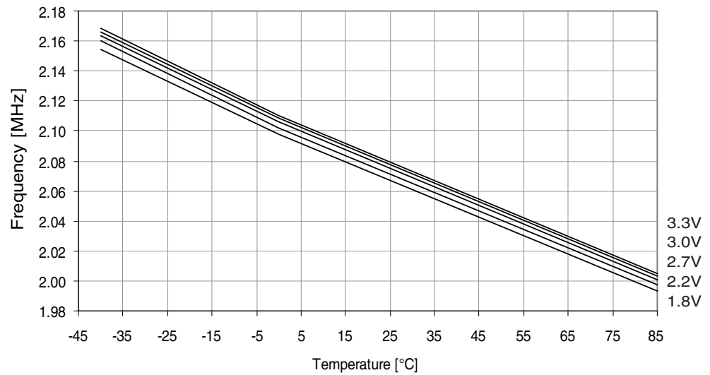
Figure 37-71. 2MHz internal oscillator frequency vs. temperature.
