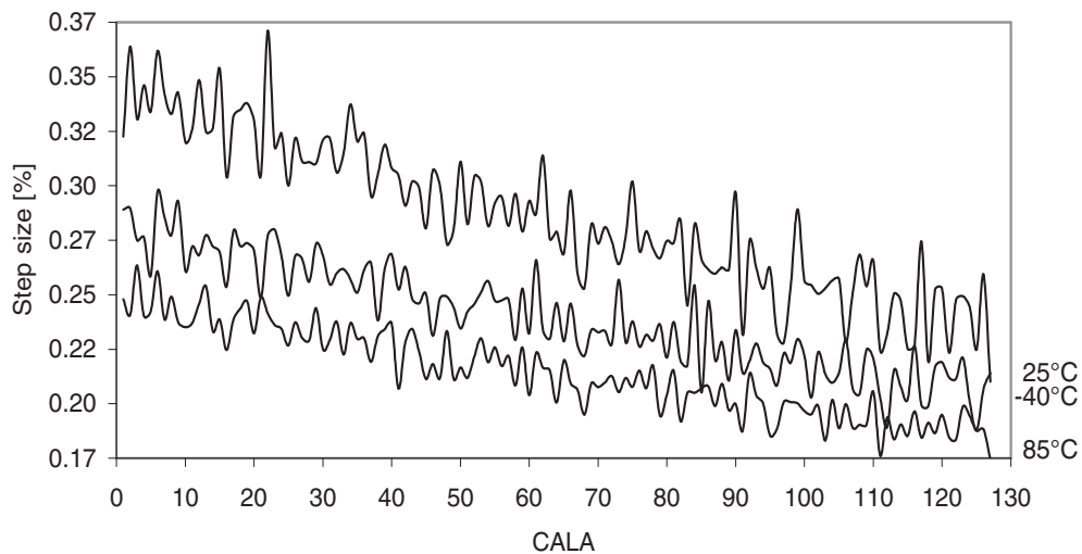
Figure 37-73. 2MHz internal oscillator CALA calibration step size.
