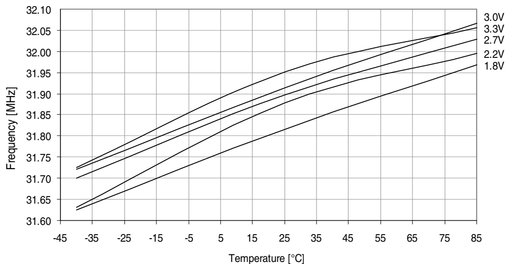
Figure 37-75. 32MHz internal oscillator frequency vs. temperature. DPLL enabled, from the 32.768kHz internal oscillator.
