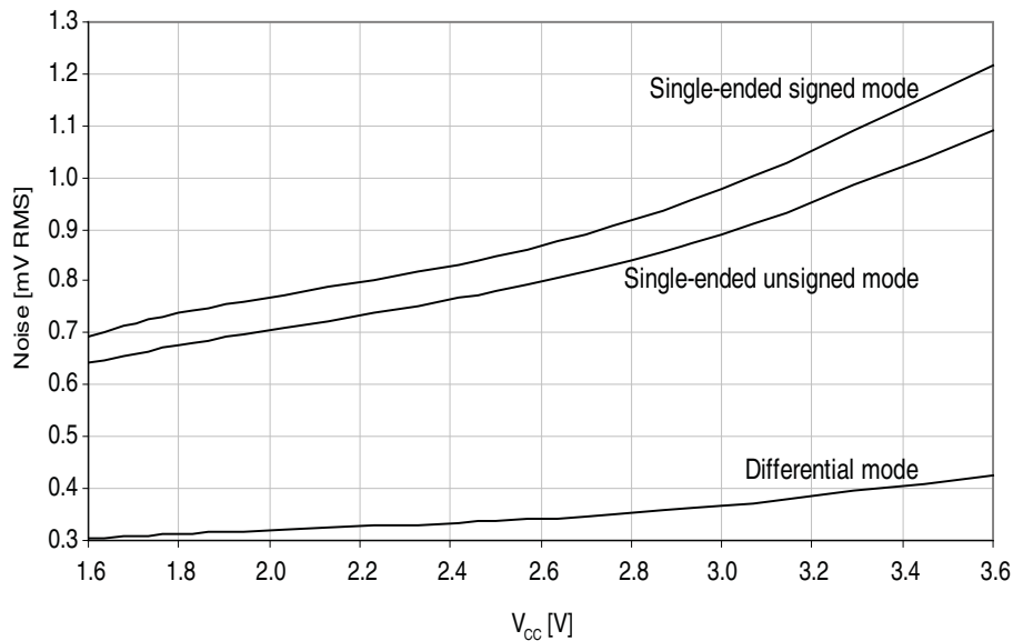
Figure 37-47. Noise vs. V_{CC} .
