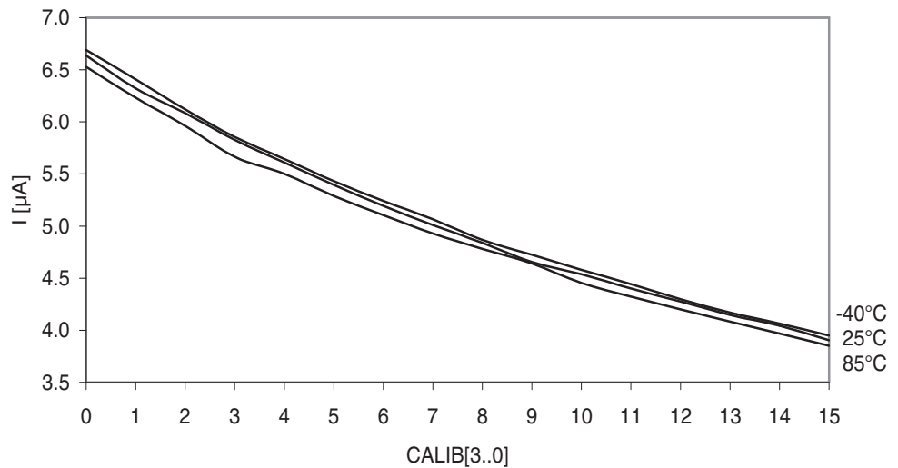
Figure 37-56. Analog comparator current source vs. calibration value.
