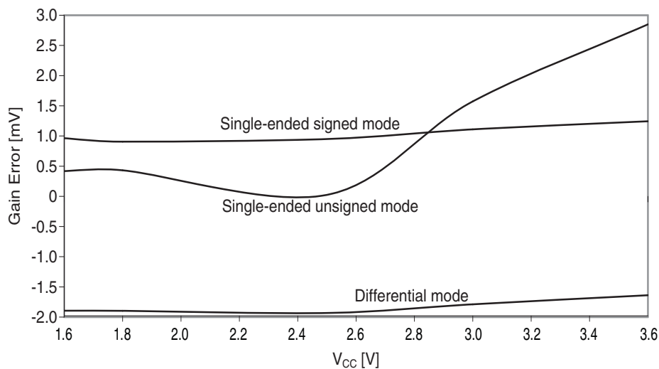
Figure 37-42. Gain error vs. V_{CC} . T = 25^{\circ}\text{C} , V_{REF} = \text{external } 1.0\text{V} , ADC sampling speed = 500ksp/s.
