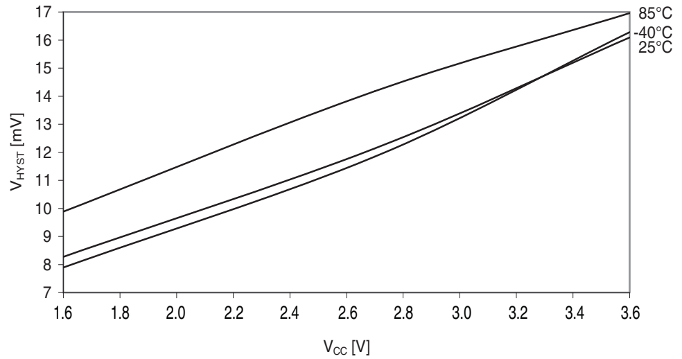
Figure 37-51. Analog comparator hysteresis vs. V_{CC} . High-speed, small hysteresis.
