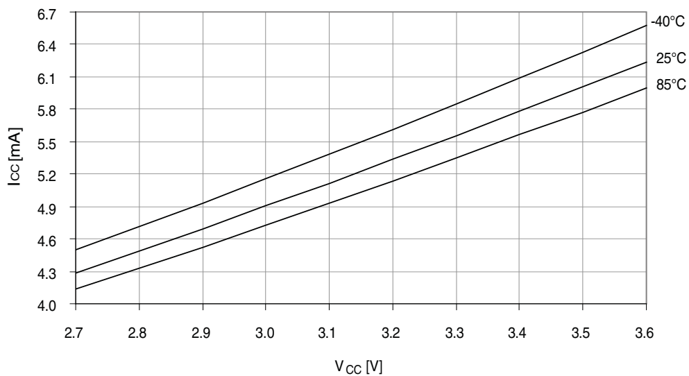
Figure 37-14. Idle mode current vs. V_{CC} . f_{SYS} = 32\text{MHz} internal oscillator.
