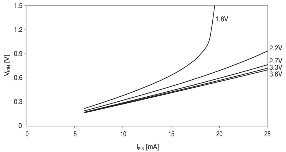
Figure 37-30. I/O pin output voltage vs. sink current.
