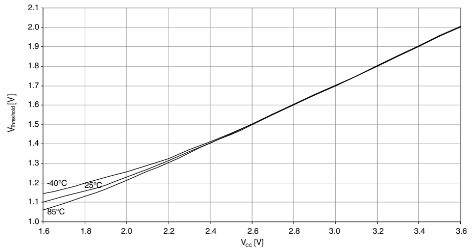
Figure 37-65. Reset pin input threshold voltage vs. V_{CC} .
