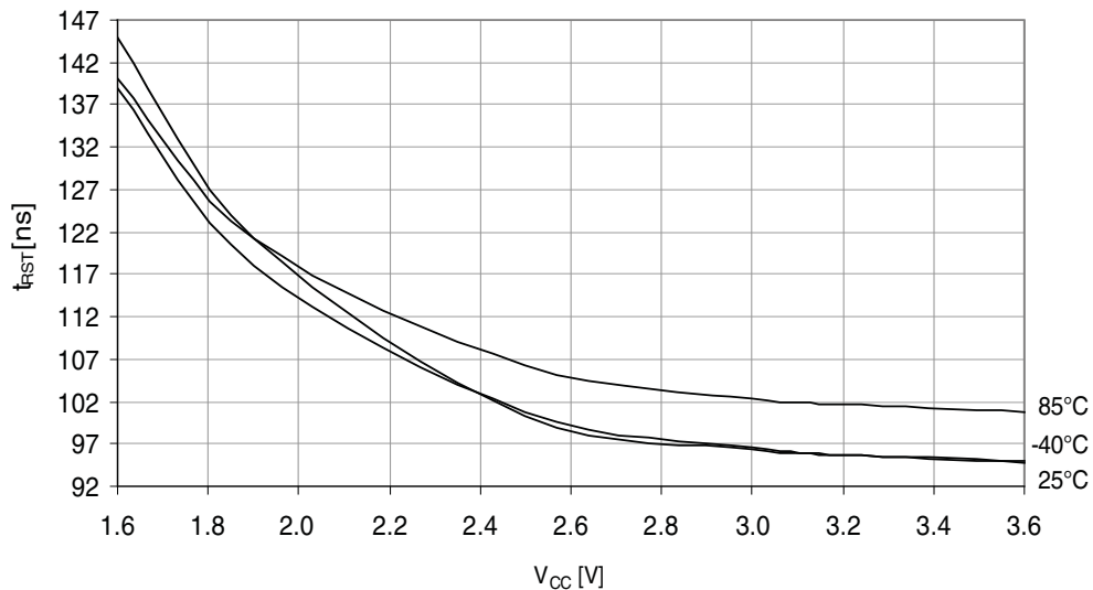
Figure 37-61. Minimum Reset pin pulse width vs. V_{CC} .
