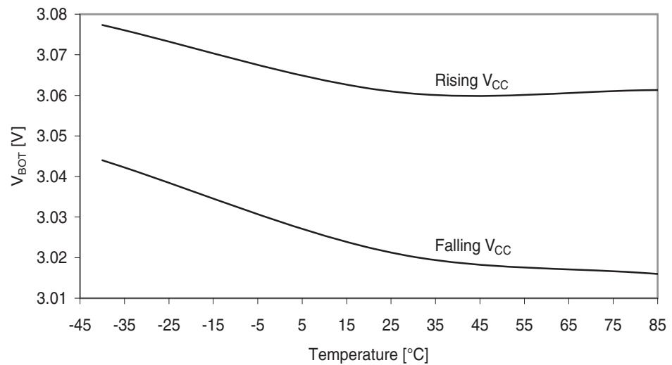
Figure 37-60. BOD thresholds vs. temperature.
