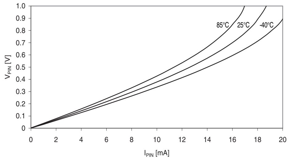
Figure 37-28. I/O pin output voltage vs. sink current.
