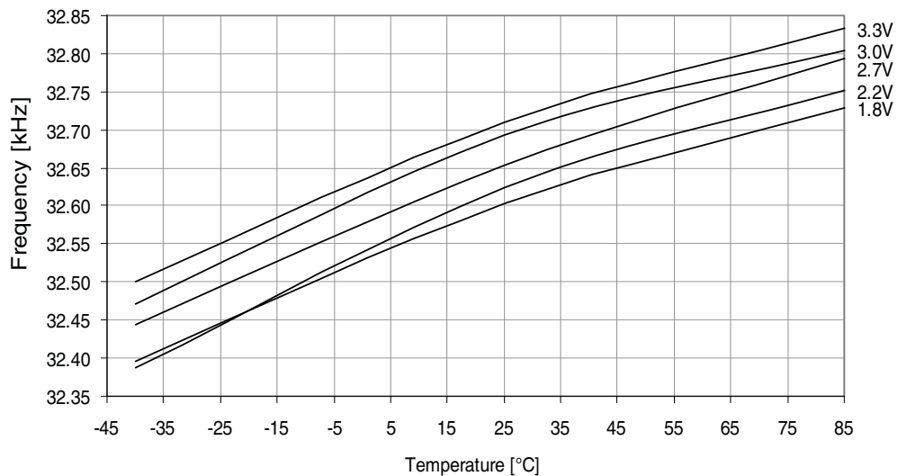
Figure 37-69. 32.768kHz internal oscillator frequency vs. temperature.
