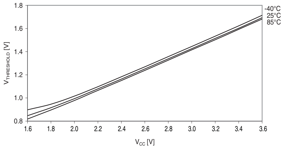
Figure 37-32. I/O pin input threshold voltage vs. V_{CC} . V_{IH} I/O pin read as "1".
