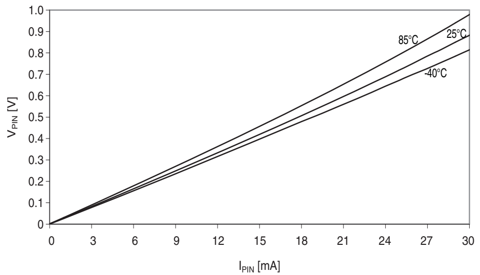
Figure 37-28. I/O pin output voltage vs. sink current.
