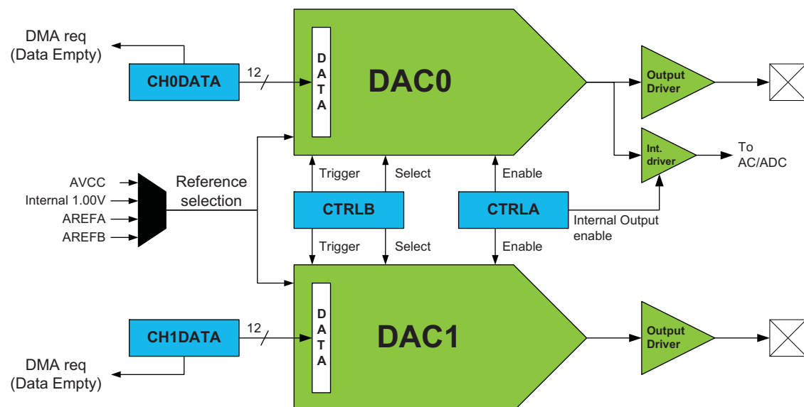
Figure 29-1. DAC overview.
