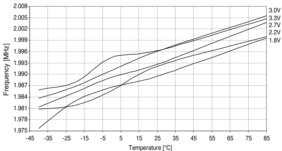
Figure 37-72. 2MHz internal oscillator frequency vs. temperature.
