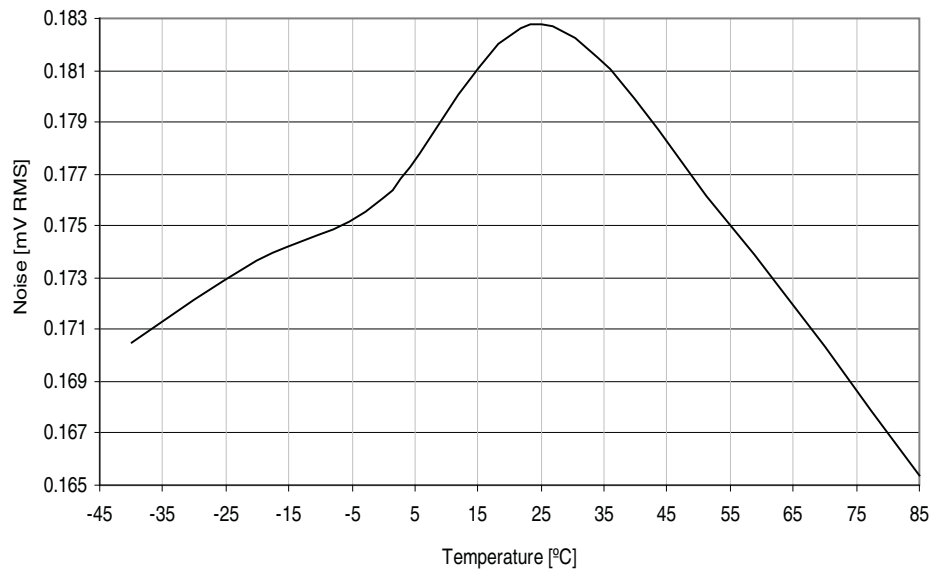
Figure 37-50. DAC noise vs. temperature.
