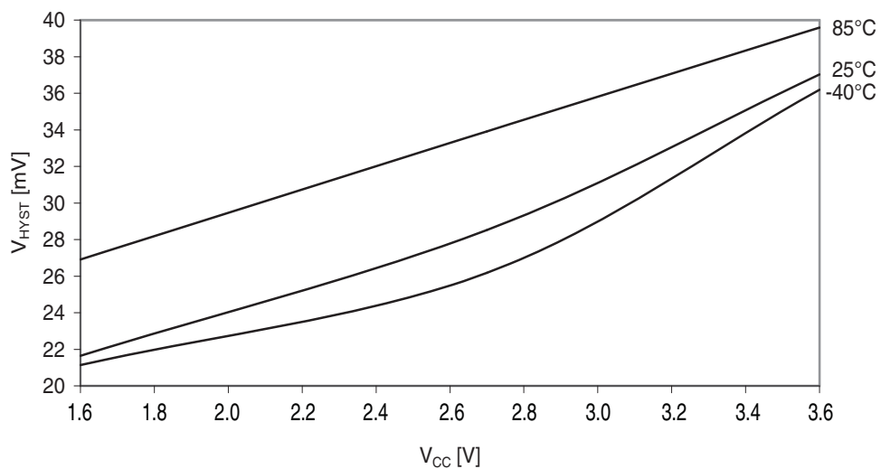
Figure 37-53. Analog comparator hysteresis vs. V_{CC} . High-speed mode, large hysteresis.
