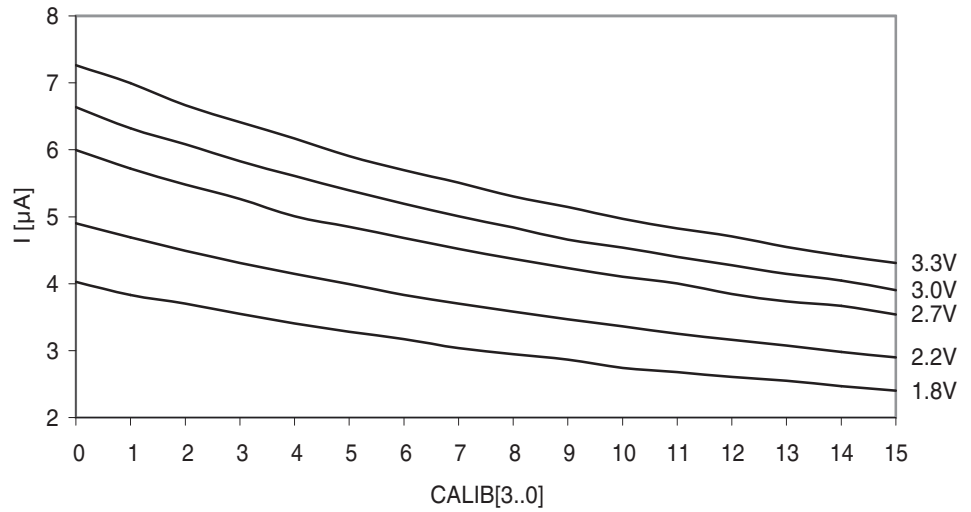
Figure 37-55. Analog comparator current source vs. calibration value.
