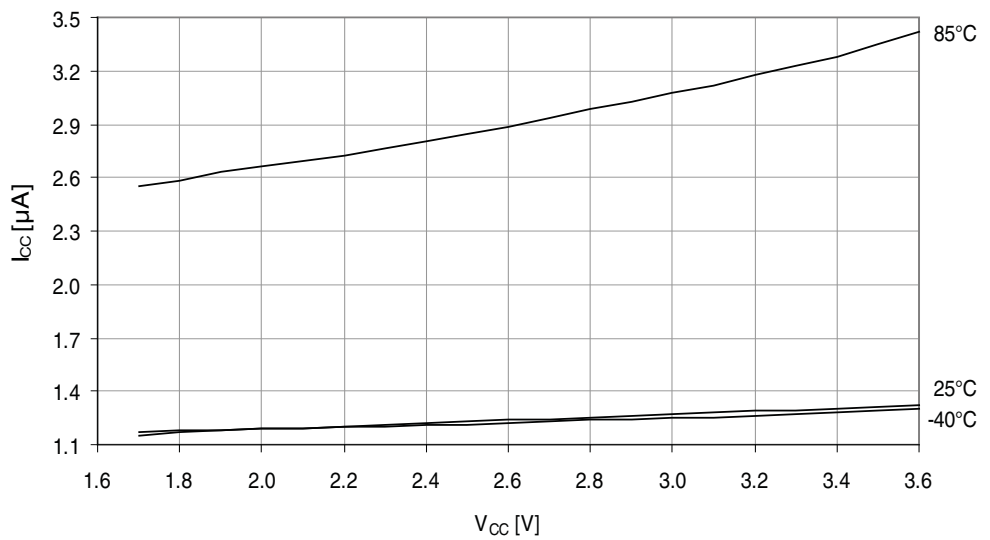
Figure 37-16. Power-down mode supply current vs. V_{CC} .
