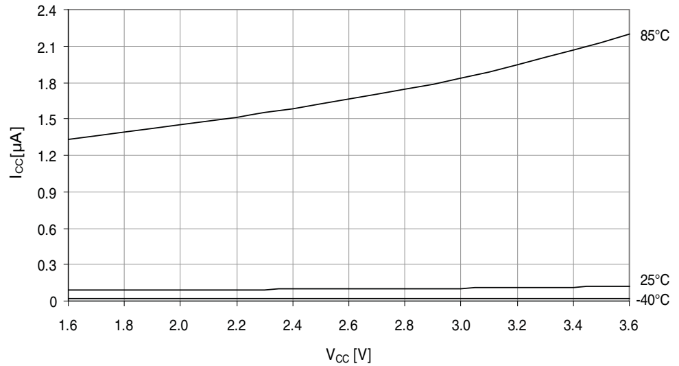
Figure 37-15. Power-down mode supply current vs. V_{CC} .
