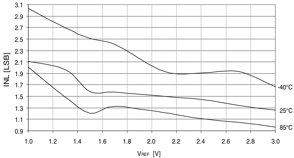
Figure 37-48. DAC INL error vs. V_{REF} .
