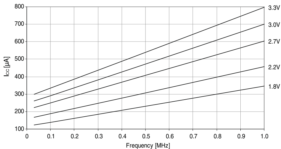
Figure 37-1. Active supply current vs. frequency.
