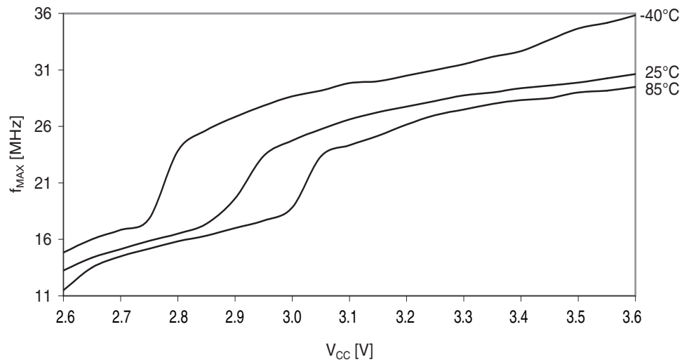
Figure 37-83. Maximum PDI frequency vs. V CC .
