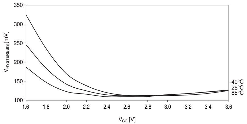
Figure 37-34. I/O pin input hysteresis vs. V_{CC} .
