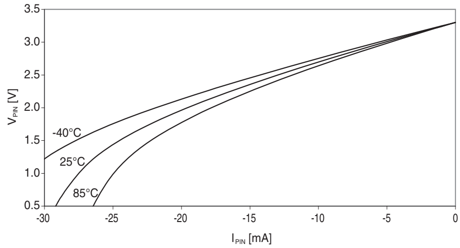
Figure 37-26. I/O pin output voltage vs. source current.
