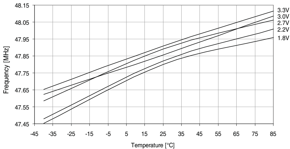
Figure 37-79. 48MHz internal oscillator frequency vs. temperature. DPLL enabled, from the 32.768kHz internal oscillator.
