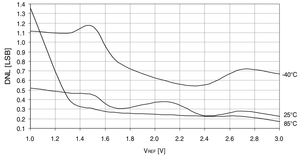
Figure 37-49. DNL error vs. V_{REF} .
