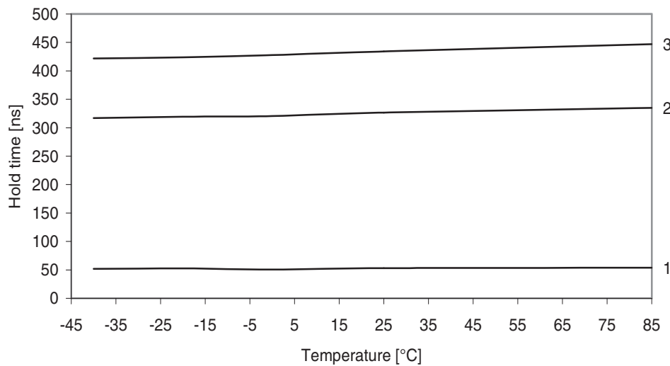
Figure 37-81. SDA hold time vs. temperature.
