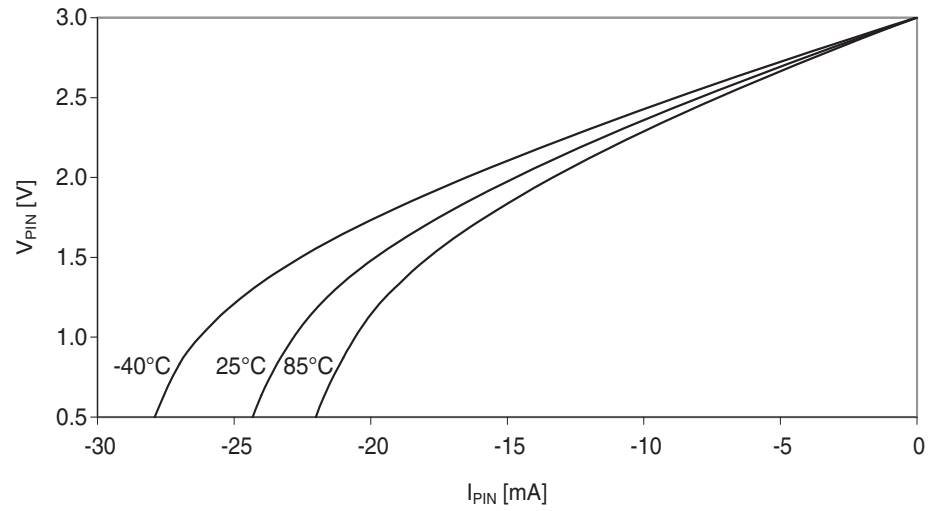
Figure 37-24. I/O pin output voltage vs. source current. V_{CC} = 3.0V .
