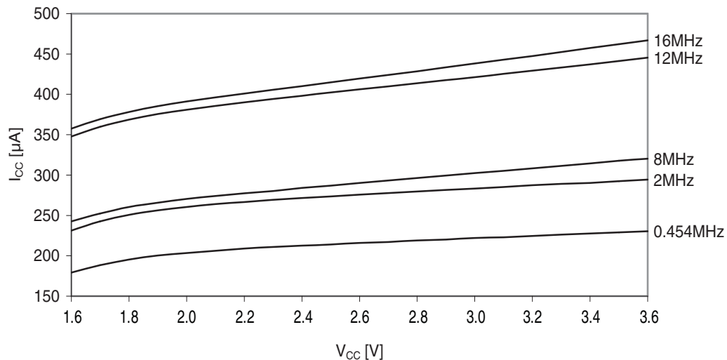
Figure 37-19. Standby supply current vs. V_{CC} . 25°C, running from different crystal oscillators.
