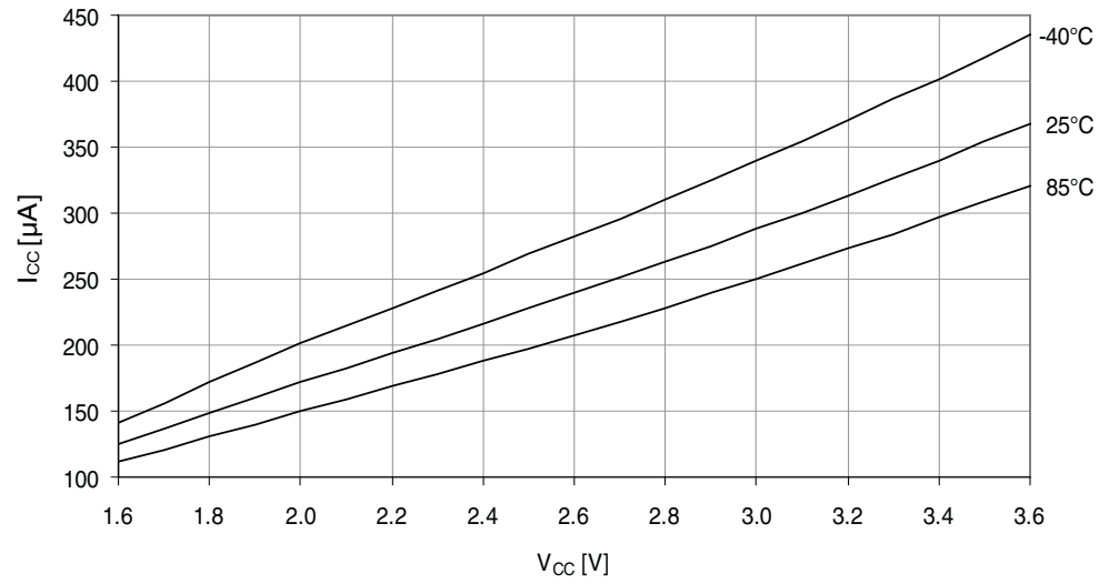
Figure 37-3. Active mode supply current vs. V_{CC} .
