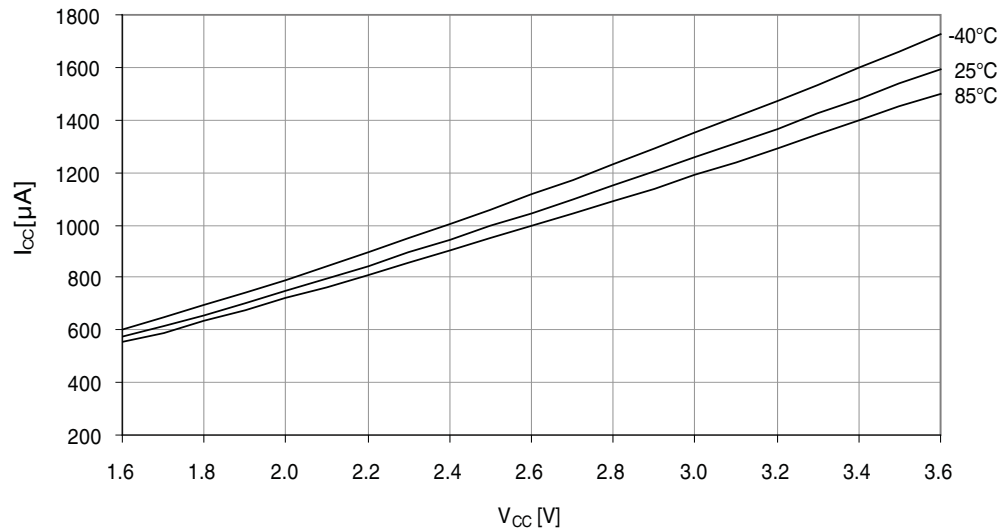
Figure 37-5. Active mode supply current vs. V_{CC} . f_{SYS} = 2MHz internal oscillator.
