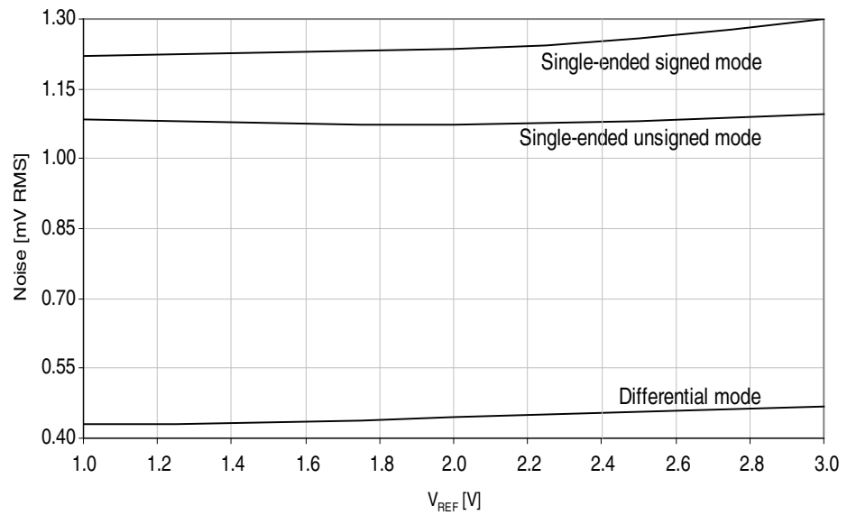
Figure 37-46. Noise vs. V_{REF} .
