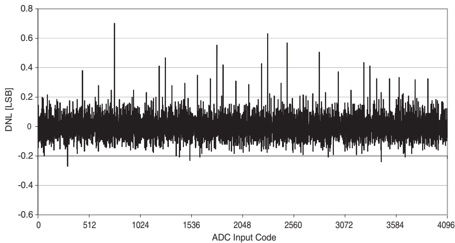
Figure 37-40. DNL error vs. input code.
