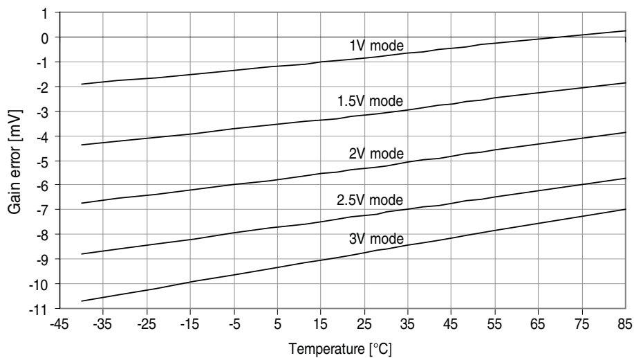
Figure 37-44. Gain error vs. temperature.
