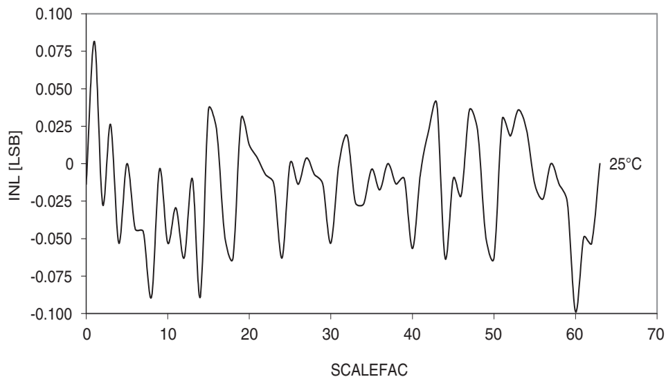
Figure 37-57. Voltage scaler INL vs. SCALEFAC.
