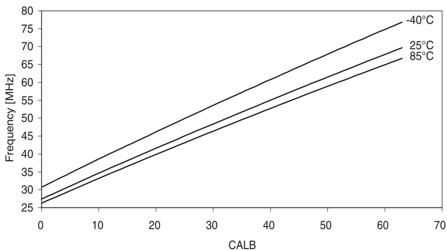
Figure 37-77. 32MHz internal oscillator frequency vs. CALB calibration value.
