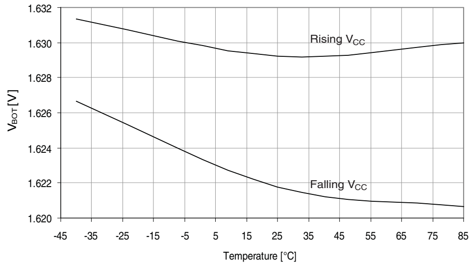
Figure 37-59. BOD thresholds vs. temperature.
