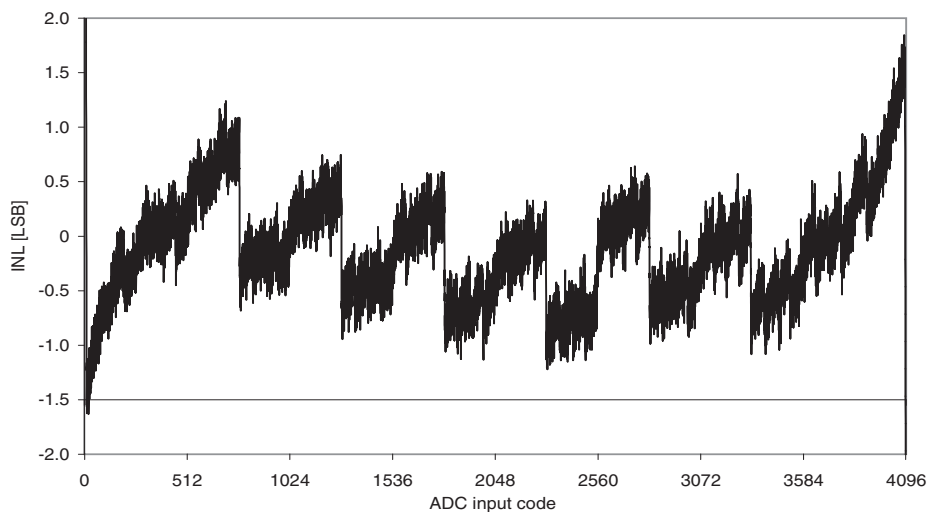
Figure 37-37. INL error vs. input code.
