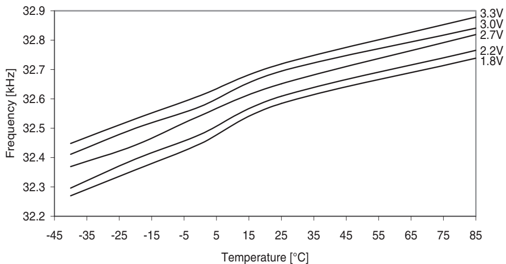
Figure 37-68. Ultra Low-Power internal oscillator frequency vs. temperature.
