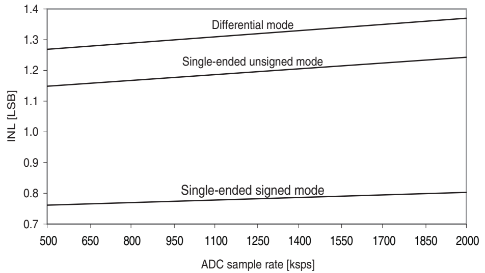
Figure 37-36. INL error vs. sample rate. T = 25°C, V_{CC} = 3.6V , V_{REF} = 3.0V external.
