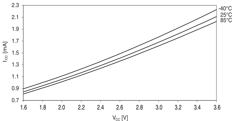
Figure 37-13. Idle mode supply current vs. V_{CC} . f_{SYS} = 32\text{MHz} internal oscillator prescaled to 8MHz.
