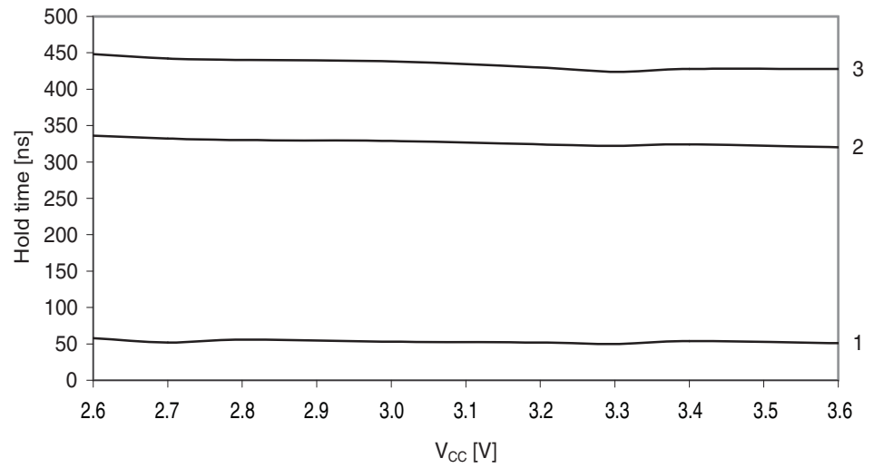
Figure 37-82. SDA hold time vs. supply voltage.
