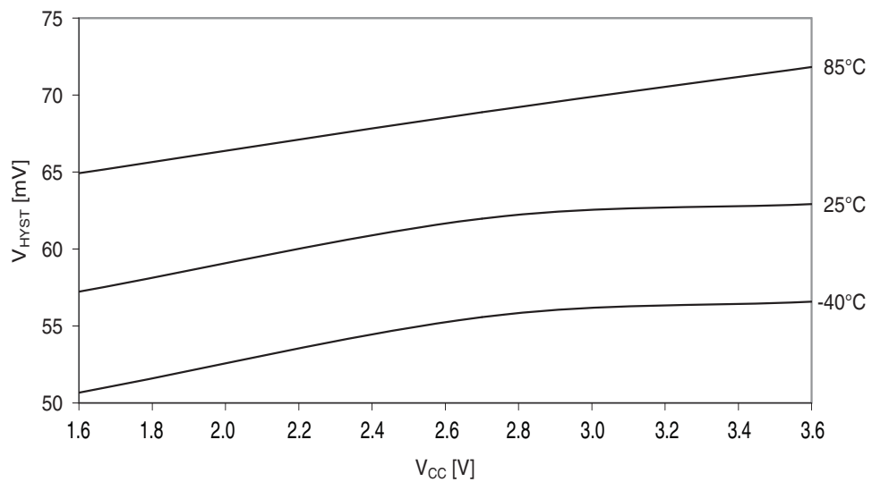
Figure 37-54. Analog comparator hysteresis vs. V_{CC} . Low power, large hysteresis.
