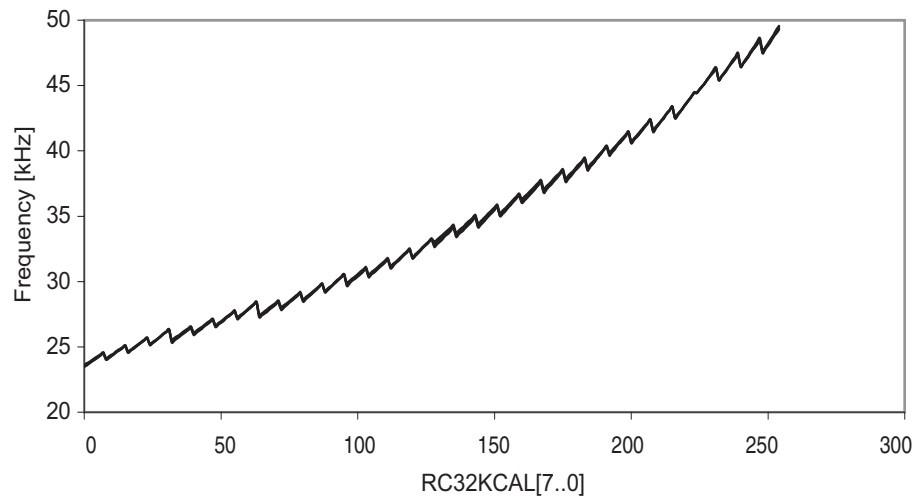
Figure 37-70. 32.768kHz internal oscillator frequency vs. calibration value.
