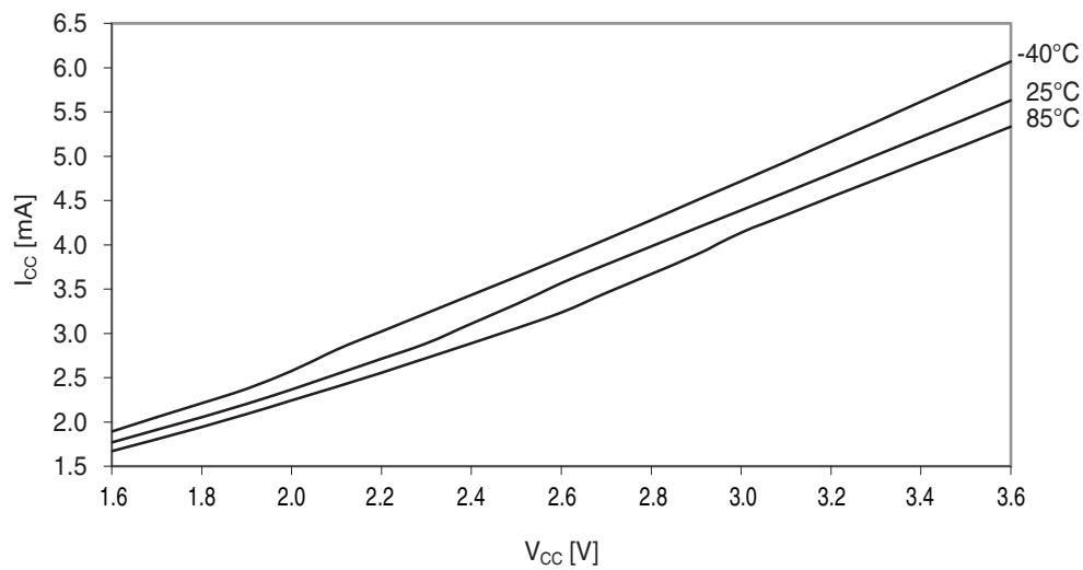
Figure 37-6. Active mode supply current vs. V_{CC} . f_{SYS} = 32MHz internal oscillator prescaled to 8MHz.
