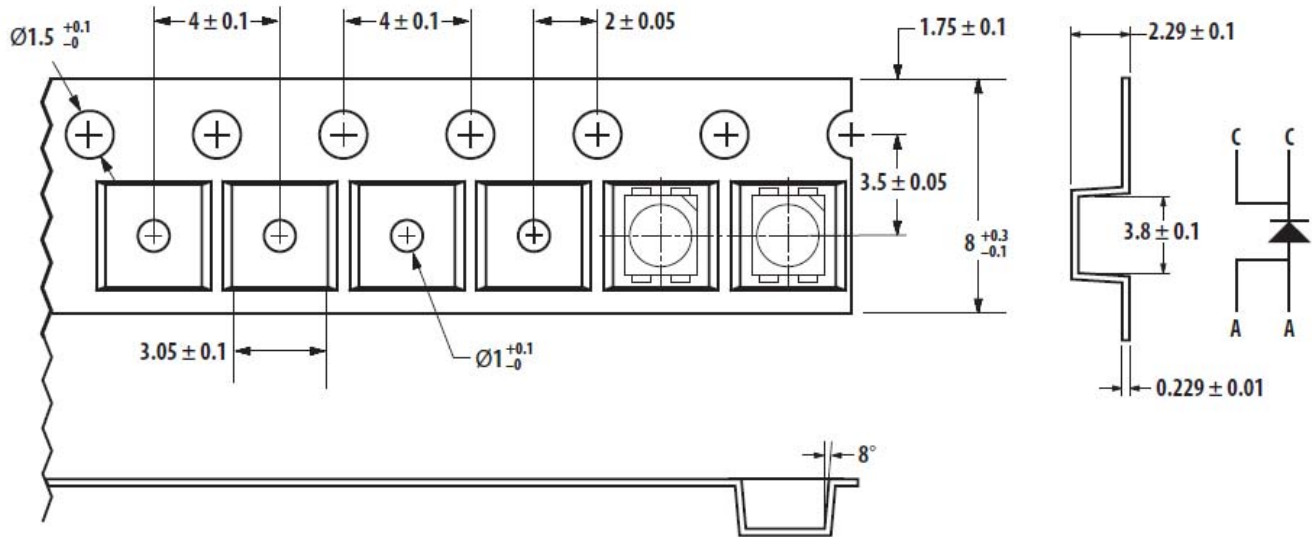
Figure 15. Tape Dimensions
