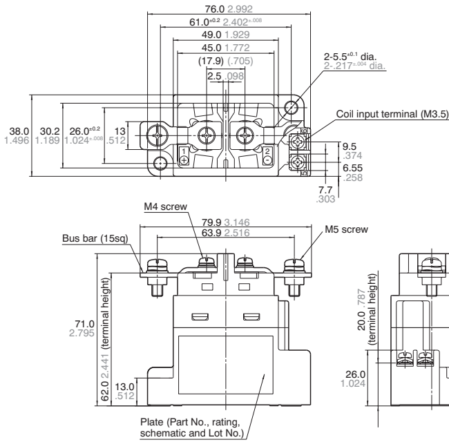
External dimensions
