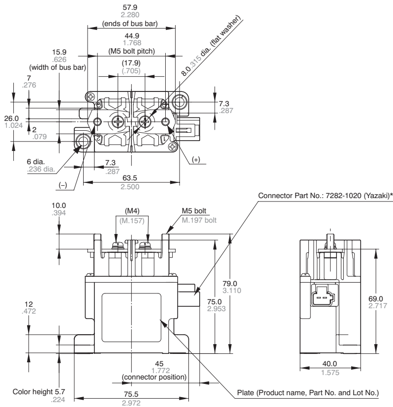
External dimensions
