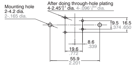
PC board pattern (Bottom view)
