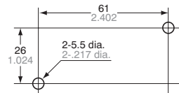
Panel cut-off
