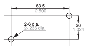
Panel cut-off
