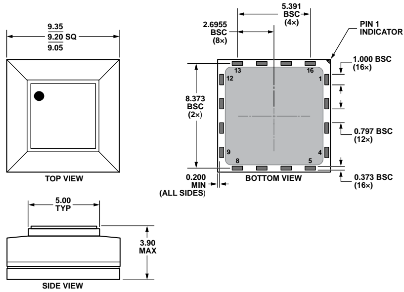
Figure 36. 16-Terminal Land Grid Array [LGA] (CC-16-2)
