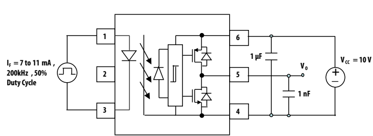
Figure 20. tr and tf test circuit and waveforms.
