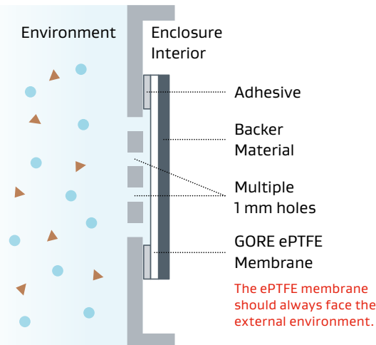
Figure 6: Interior mounting is recommended for Parts Series VE8
