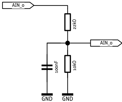
Figure 3.4 Internal circuit of AIN_0
