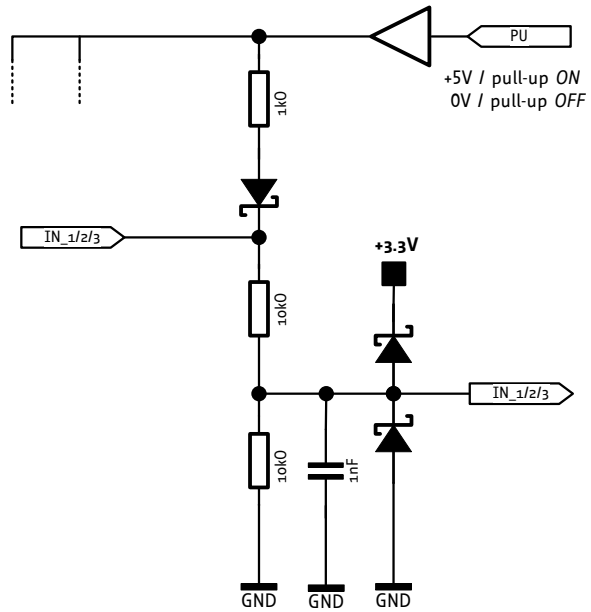
Figure 3.5 Internal circuit of IN_1/2/3
