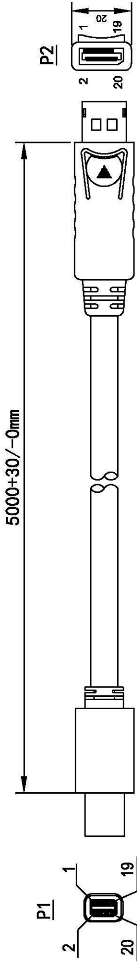
DisplayPort Male
