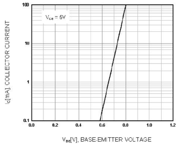
Figure 2. Transfer Characteristic
