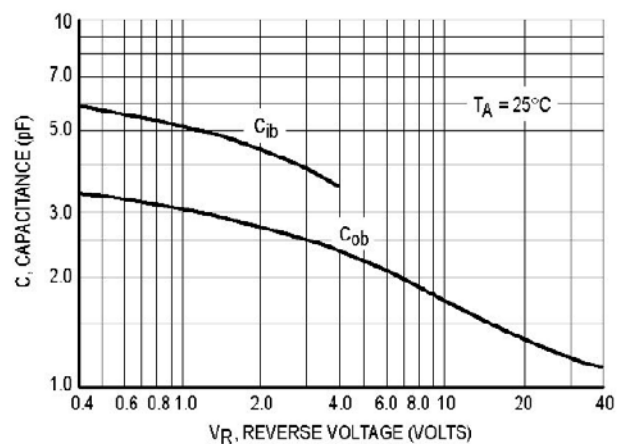
Figure 4. Capacitances
