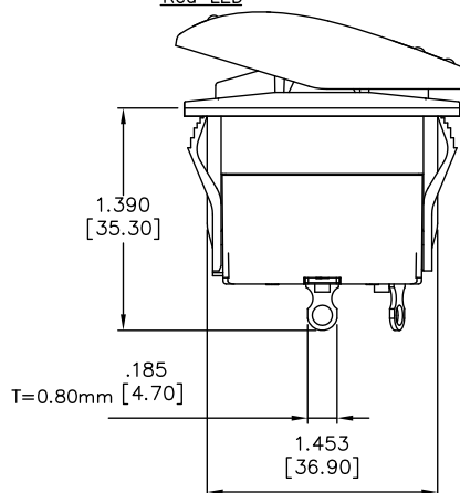
POS. 1 Red LED POS. 2
