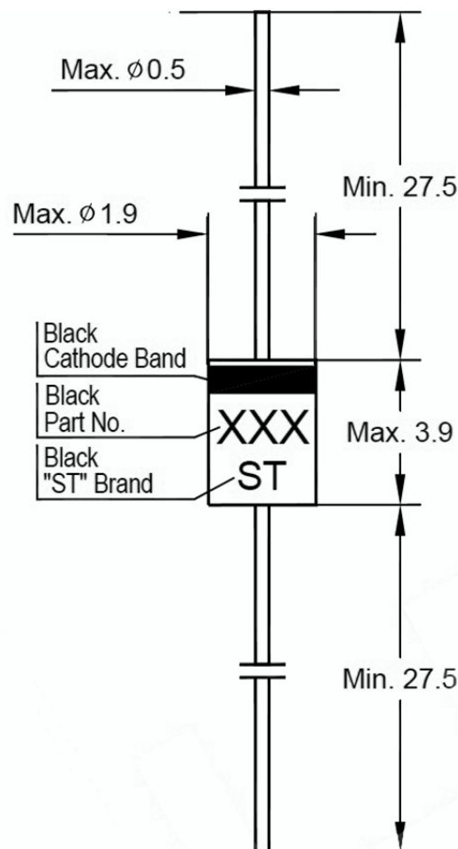
Glass Case DO-35 Dimensions in mm
