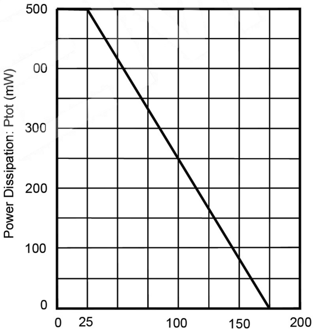
Ambient Temperature: T_a (°C) Power Derating Curve
