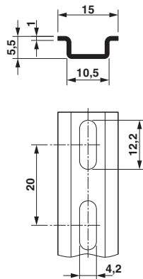
Dimensional drawing
