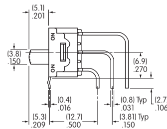
Actuator in LEFT Position
