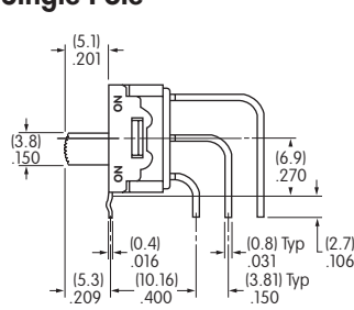
Actuator in LEFT Position
