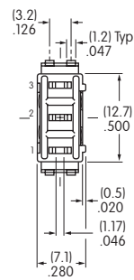
Actuator in LEFT Position
