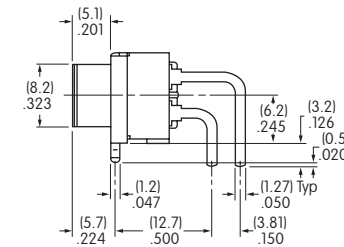
Actuator in LEFT Position
