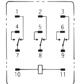
Terminal Arrangement/ Internal Connections (Bottom View) Standard Models
