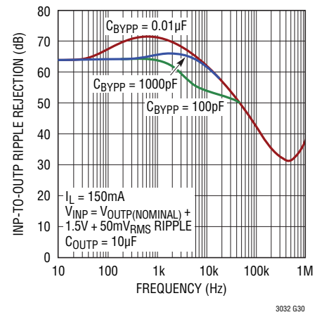
INP-to-OUTP Ripple Rejection
