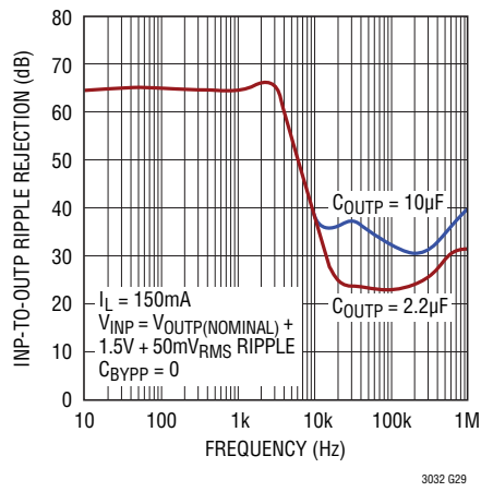
INP-to-OUTP Ripple Rejection
