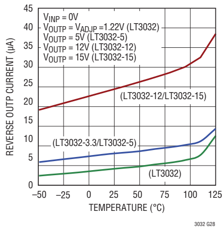
Reverse OUTP Pin Current
