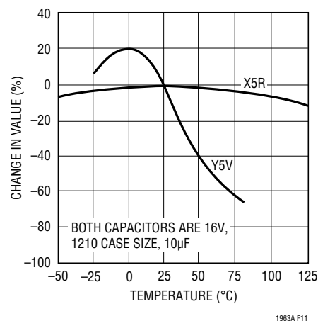
Figure 11. Ceramic Capacitor Temperature Characteristics
