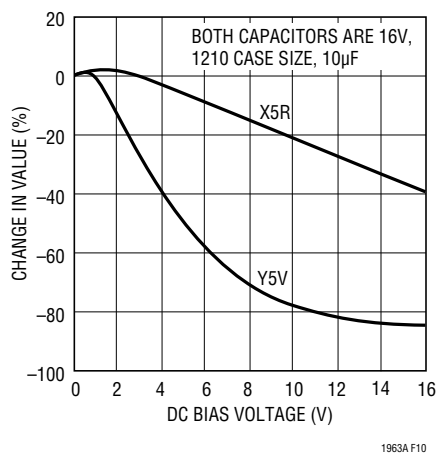
Figure 10. Ceramic Capacitor DC Bias Characteristics
