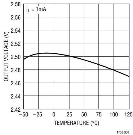
LT1764A-2.5 Output Voltage
