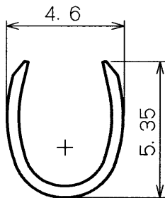
B-B sec.
