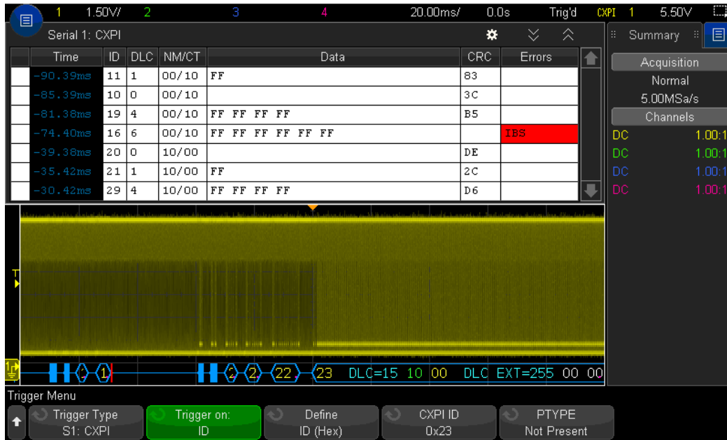
Figure 9. CXPI decode on an InfiniiVision X-Series oscilloscope.
