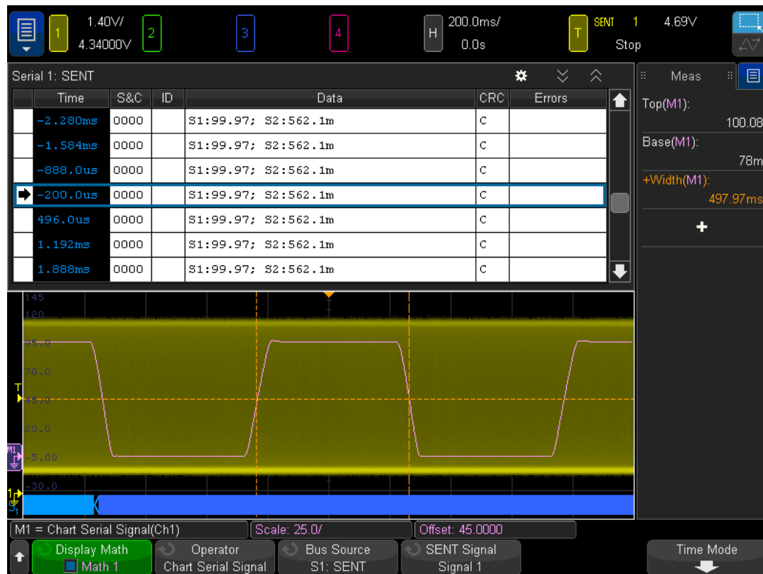
Figure 2. SENT-based throttle blade position signal (S1) charted on the oscilloscope's display.
