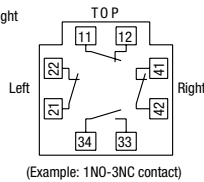
(Example: 1NO-3NC contact)
