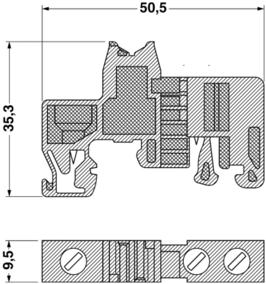
Dimensional drawing
