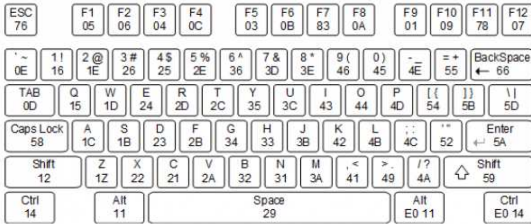
( https://reference.digilentinc.com/_detail/reference/programmable-logic/nexys-a7/n4k.png?id=reference%3Aprogrammable-logic%3Anexys-a7%3Areference-manual ) Figure 7.2.1 Keyboard Scan Codes
