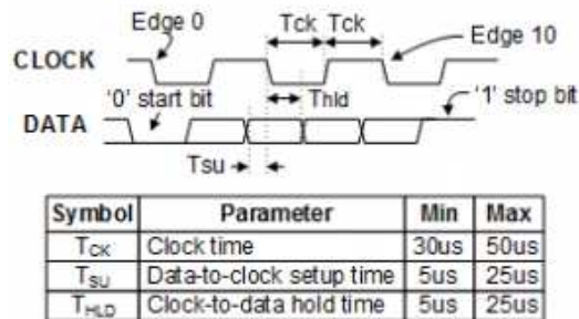
( https://reference.digilentinc.com/_detail/reference/programmable-logic/nexys-a7/n4j.png?id=reference%3Aprogrammable-logic%3Anexys-a7%3Areference-manual ) Figure 7.1.1 PS/2 Device-to-Host Timing Diagram
