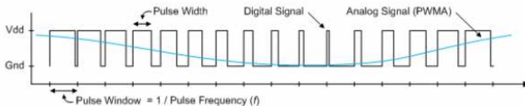
( https://reference.digilentinc.com/_detail/reference/programmable-logic/nexys-a7/n4ag.png?id=reference%3Aprogrammable-logic%3Anexys-a7%3Areference-manual ) Figure 15.1.1 Simple Waveform Represented as PWM
