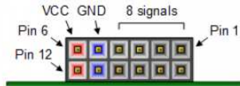
( https://reference.digilentinc.com/_detail/reference/programmable-logic/nexys-a7/n4v.png?id=reference%3Aprogrammable-logic%3Anexys-a7%3Areference-manual ) Figure 10.1 Pmod Connectors; Front View, as Loaded on PCB
