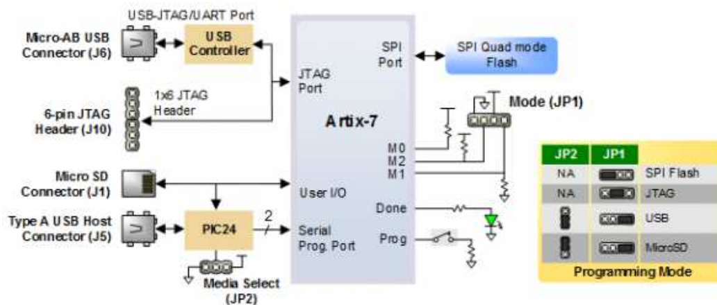
( https://reference.digilentinc.com/_detail/reference/programmable-logic/nexys-a7/n4e.png?id=reference%3Aprogrammable-logic%3Anexys-a7%3Areference-manual ) Figure 2.1 Nexys A7 DDR Configuration Options
