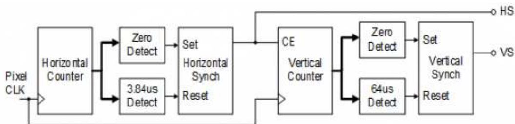
( https://reference.digilentinc.com/_detail/reference/programmable-logic/nexys-a7/n4q.png?id=reference%3Aprogrammable-logic%3Anexys-a7%3Areference-manual ) Figure 8.1.4 VGA Display Controller Block Diagram
