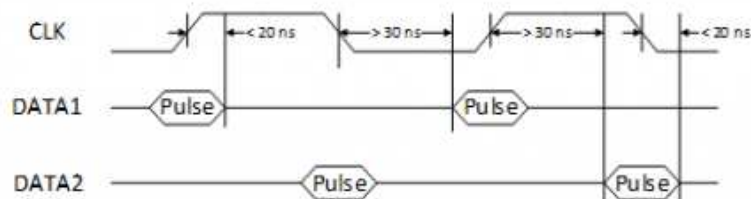
( https://reference.digilentinc.com/_detail/reference/programmable-logic/nexys-a7/n4ac.png?id=reference%3Aprogrammable-logic%3Anexys-a7%3Areference-manual ) Figure 14.2.1 PDM Timing Diagram
