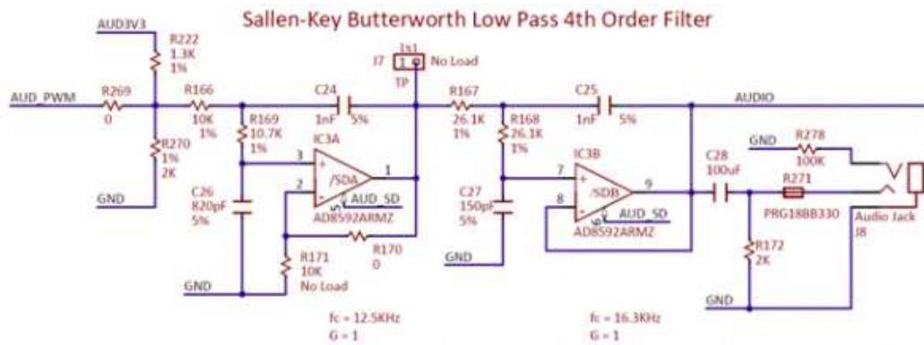
( https://reference.digilentinc.com/_detail/reference/programmable-logic/nexys-a7/n4ae.png?id=reference%3Aprogrammable-logic%3Anexys-a7%3Areference-manual ) Figure 15.1 Sallen-Key Butterworth Low-Pass 4th Order Filter
