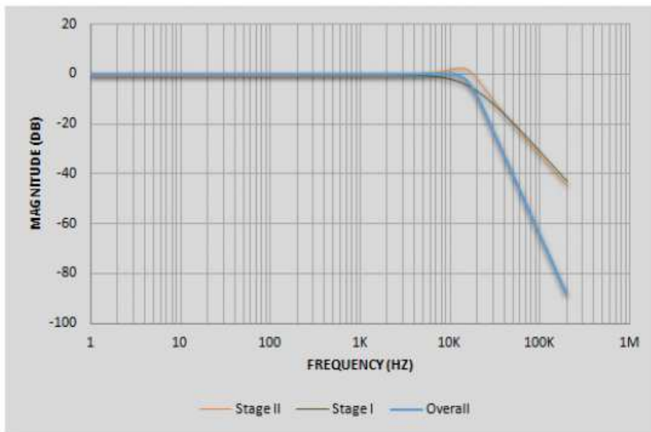
( https://reference.digilentinc.com/_detail/reference/programmable-logic/nexys-a7/n4af.png?id=reference%3Aprogrammable-logic%3Anexys-a7%3Areference-manual ) Figure 15.2 SK Butterworth Low-Pass Filter Frequency Response
