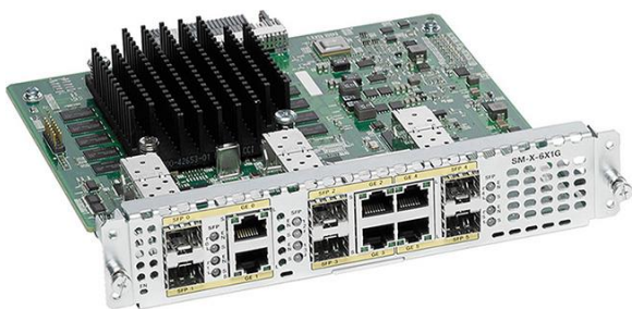
Figure 2. Cisco 6-Port High-Density Gigabit Ethernet WAN Service Module
